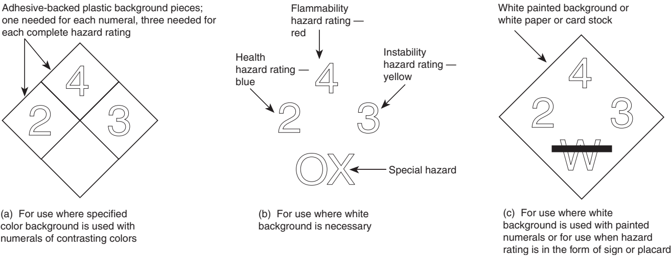
FIGURE 9.1(a) Alternative Arrangements for Display of NFPA 704 Hazard Identification System.
