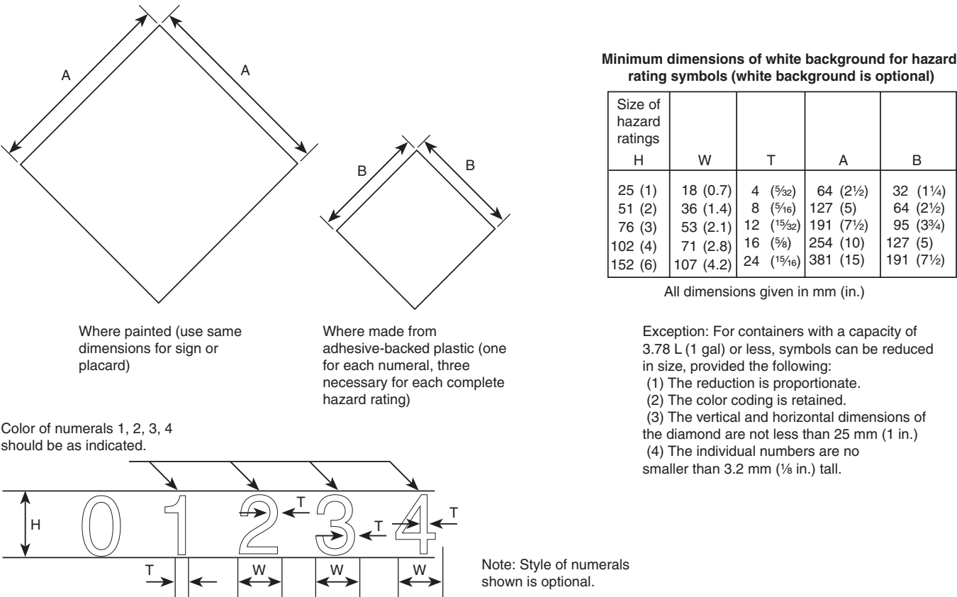
FIGURE 9.1(b) Dimensions of NFPA 704 Placard and Numerals.
