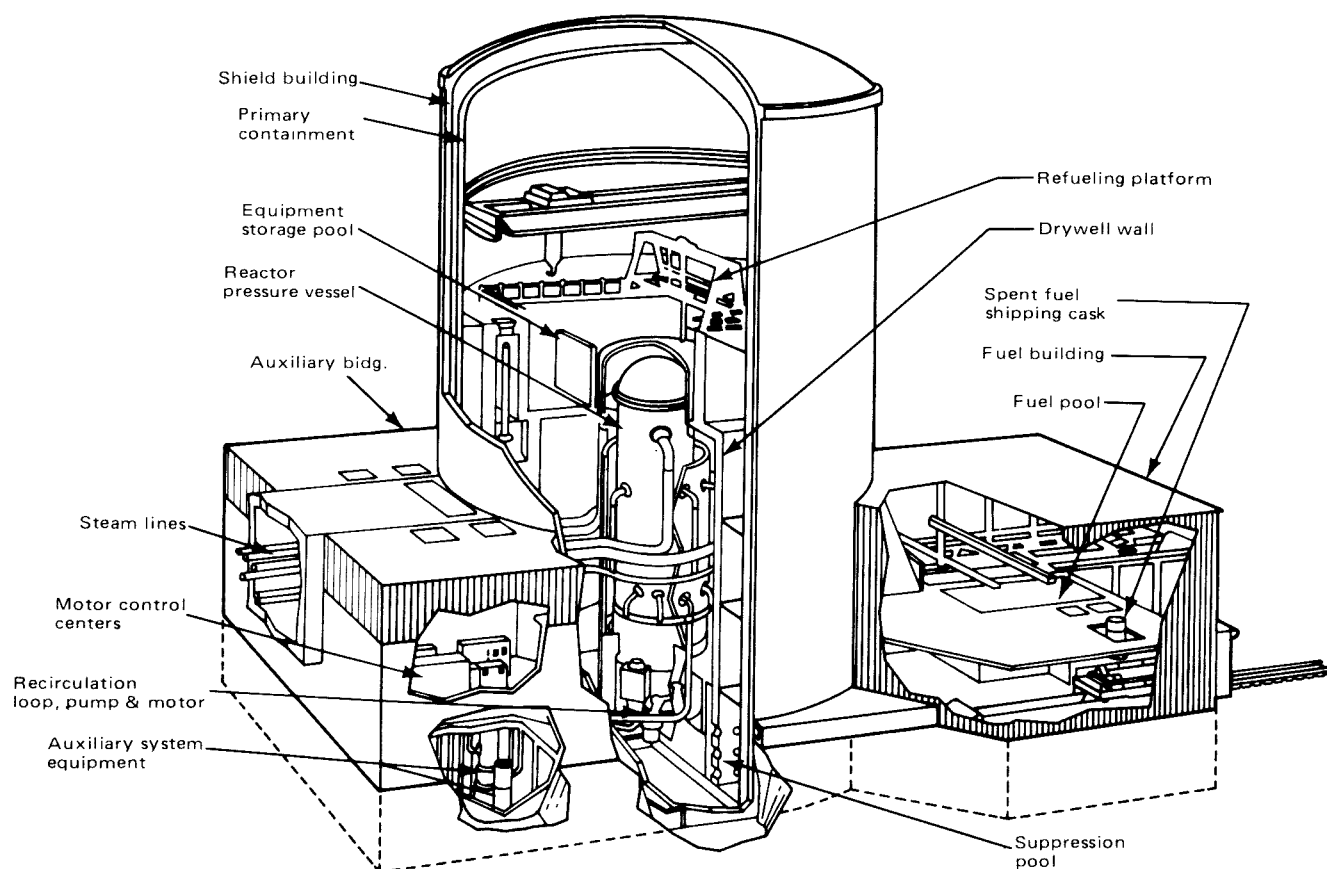
Figure 2-1 Mark III reactor building, fuel building, and auxiliary building.
