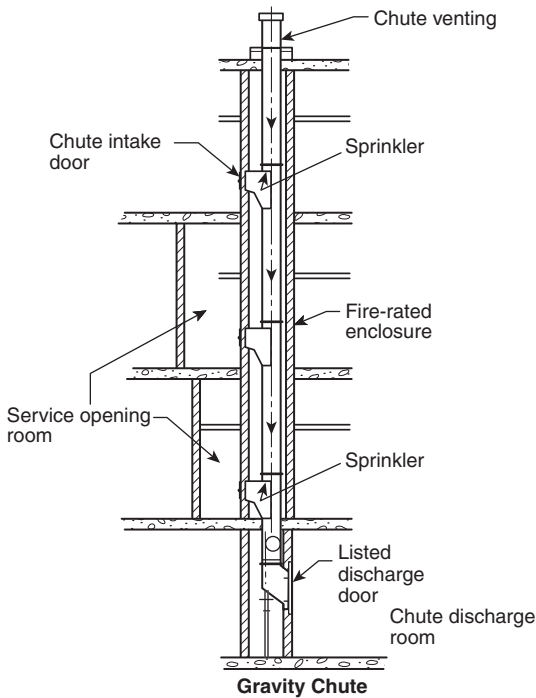
FIGURE A.6.2(a) Gravity Linen Chute.
