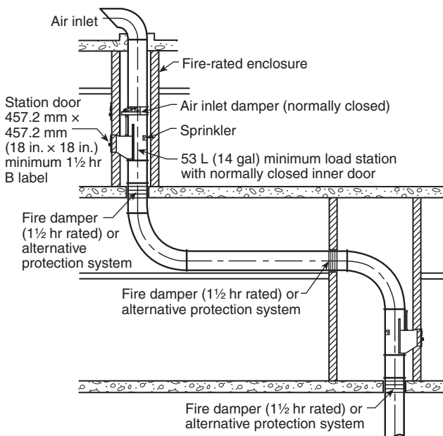
▲ FIGURE 6.3.5.2.1(a) Full Pneumatic Riser with Offset.
