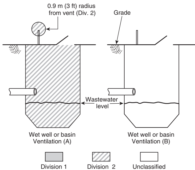
FIGURE A.4.2(b) Wet Well or Basin Serving a Residential Sewer; Illustration of Table 4.2.2, Row 11.
