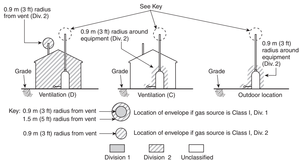
FIGURE A.4.2(g) Odor-Control System Location Physically Separated from Wet Well; Illustration of Table 4.2.2, Row 20.
