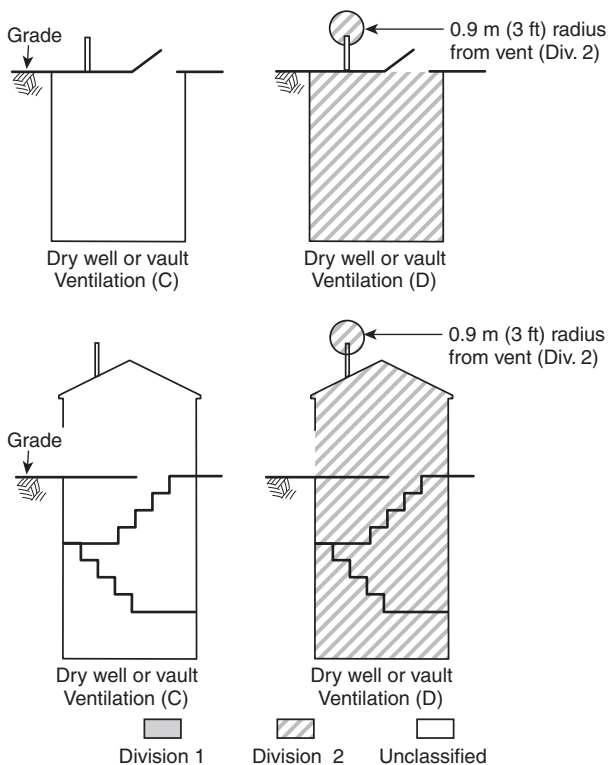
FIGURE A.4.2(e) Belowgrade or Partially Belowgrade Equipment Housing or Vault Physically Separated from Wet Well or Basin; Illustration of Table 4.2.2, Rows 5, 12, 17, 31, and 36.
