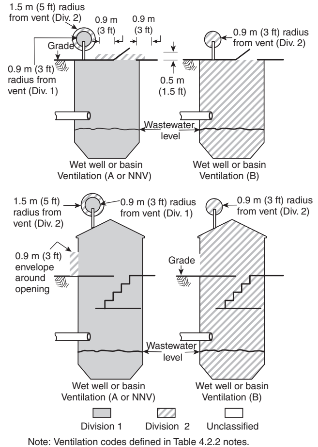
FIGURE A.4.2(c) Wet Well or Basin Serving Separate or Combined Sanitary Sewer; Illustration of Table 4.2.2, Rows 16 and 34.
