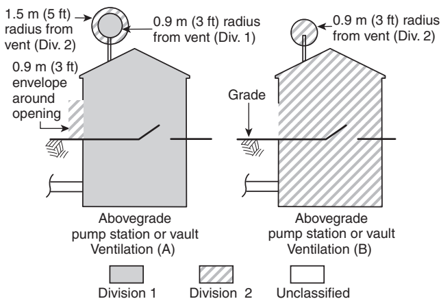
FIGURE A.4.2(f) Abovegrade Equipment Housing or Vault not Physically Separated from Wet Well or Basin; Illustration of Table 4.2.2, Row 19.
