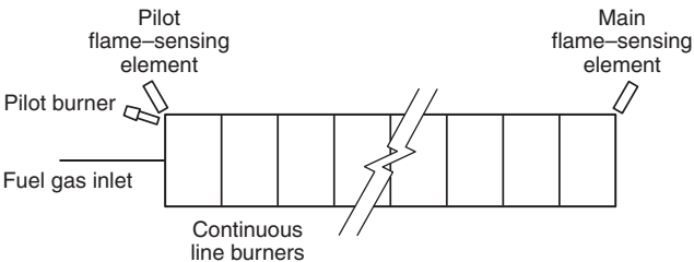
FIGURE A.8.10.2.2(a) Example of a Combustion Safeguard Supervising a Pilot for a Continuous Line Burner During Light-Off and the Main Flame Alone During Firing.
