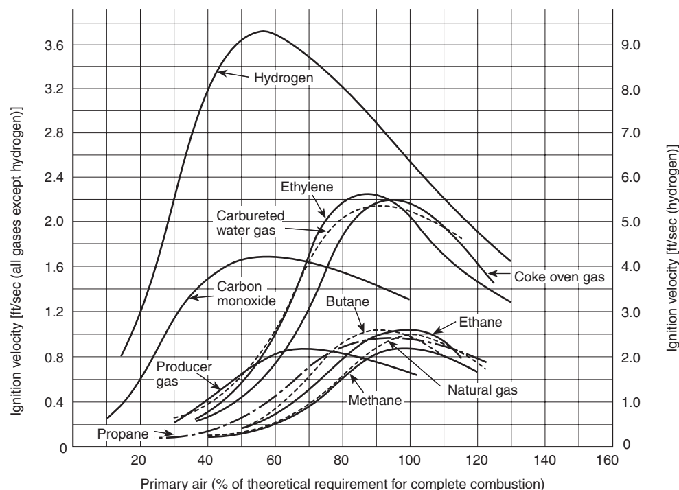
FIGURE A.6.2 Ignition Velocity Curves for Typical Flammable Gases.
