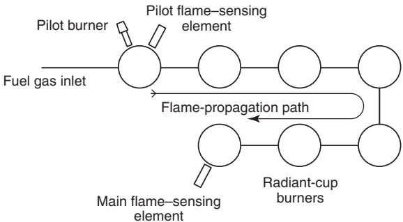
FIGURE A.8.10.2.2(b) Example of a Combustion Safeguard Supervising a Group of Radiant Cup Burners Having Reliable Flame-Propagation Characteristics from One to the Other by Means of Flame-Propagation Devices.
