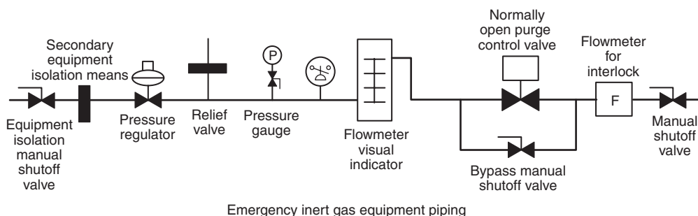
FIGURE A.13.5.11.10 Examples of Special Atmosphere Equipment Piping.
