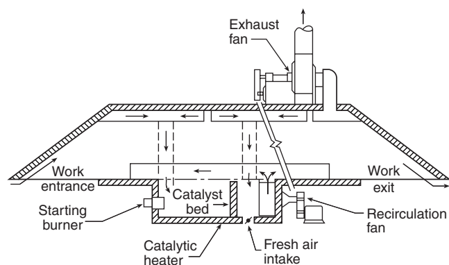
FIGURE A.10.6.4(b) Example of Indirect-Type Catalytic Oven Heater for Full Air Pollution Control.
