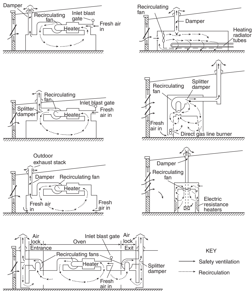
FIGURE A.11.6.1.10 Unacceptable Safety Ventilation Systems Using a Single Fan (Recirculation Combined with Spill Exhaust).
