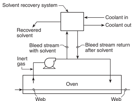
FIGURE A.11.7.1.2 Example of a Low-Oxygen Oven with a Solvent Recovery System.
