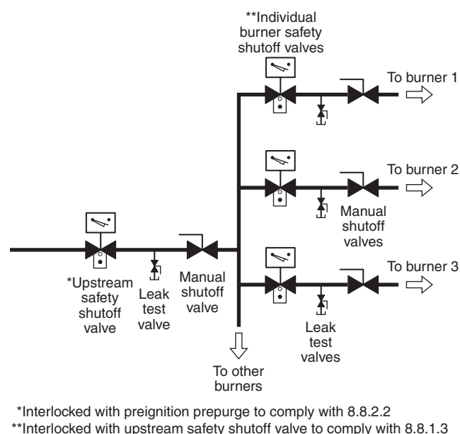
FIGURE A.8.8.1.2 Multiple Burner System Using Proof-of-Closure Switches.
