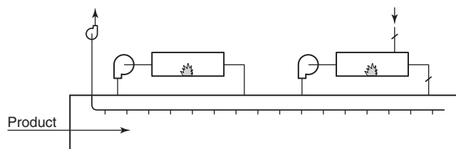
FIGURE A.11.6.10.3(b) Two Heating Zones — Common Exhaust Fan with Internal Exhaust Plenum.
