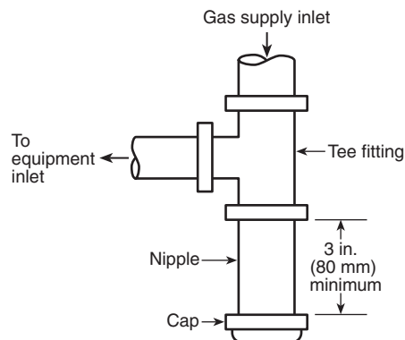
FIGURE 6.2.5.2 Method of Installing a Tee Fitting Sediment Trap. [54:Fig. 9.6.7]
