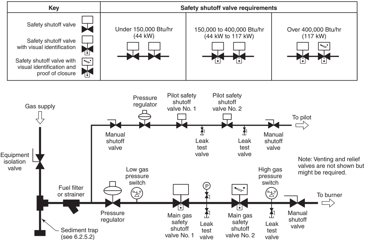
FIGURE A.8.8.2 Typical Piping Arrangement Showing Fuel Gas Safety Shutoff Valves.
