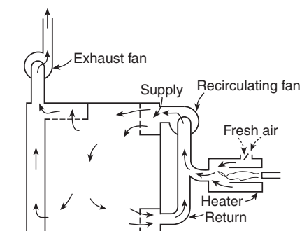
FIGURE A.3.3.30.3(c) Example of a Direct-Fired, External, Recirculating-Not-Through Heater.
