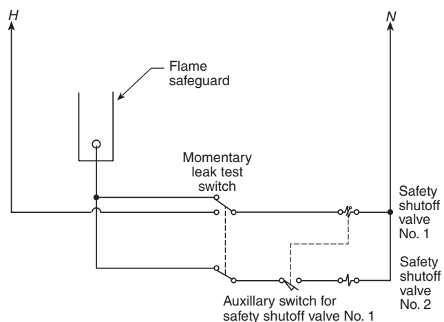
FIGURE A.7.5.14(b) Example of a Wiring Diagram for Leak Test. [86:Figure A.7.4.9(b)]
