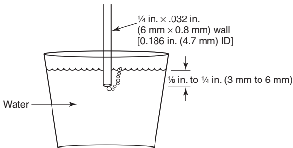
Δ FIGURE A.7.5.14(c) Leak Test for a Safety Shutoff Valve. [86:Figure A.7.4.9(c)]
