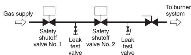
FIGURE A.7.5.14(a) Example of a Gas Piping Diagram for Leak Test. [86:Figure A.7.4.9(a)]
