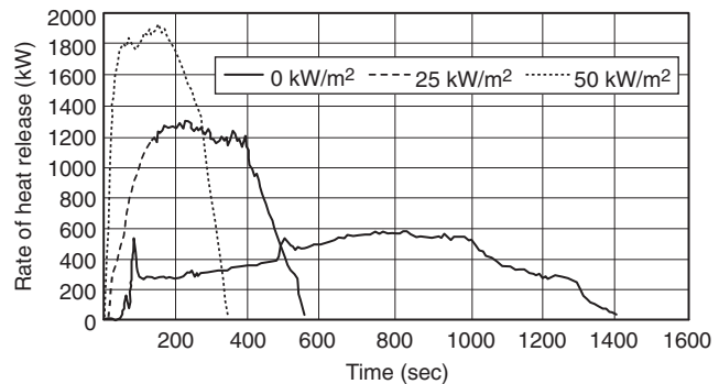
FIGURE B.6.2 Typical Graphic Output of Cone Calorimeter Test.
