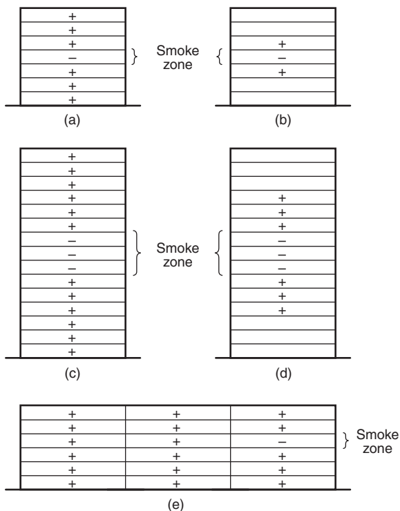
FIGURE A.4.8.1.1.1 Arrangements of Smoke Control Zones.
