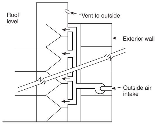
FIGURE F.4 Stairwell Pressurization with Vent to the Outside.
