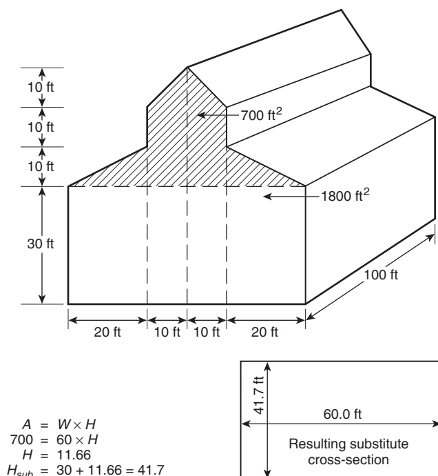
FIGURE E.3.1(a) Large Space with Nonflat Ceiling.
