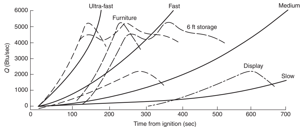
FIGURE C.2(b) Rates of Energy Release in a t -squared Fire.
