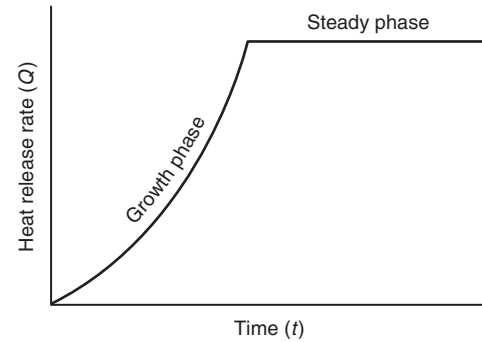
FIGURE 5.2.4(a) Unsteady Design Fire with Steady Phase.
