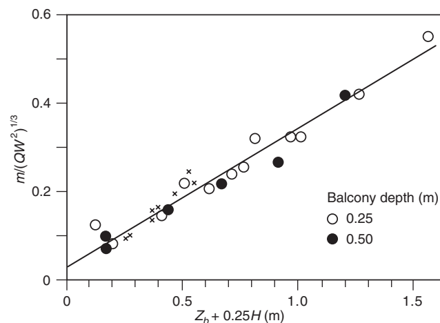
FIGURE A.6.2.2.1 Agreement Between Predictions and Experimental Values [60, 64].
