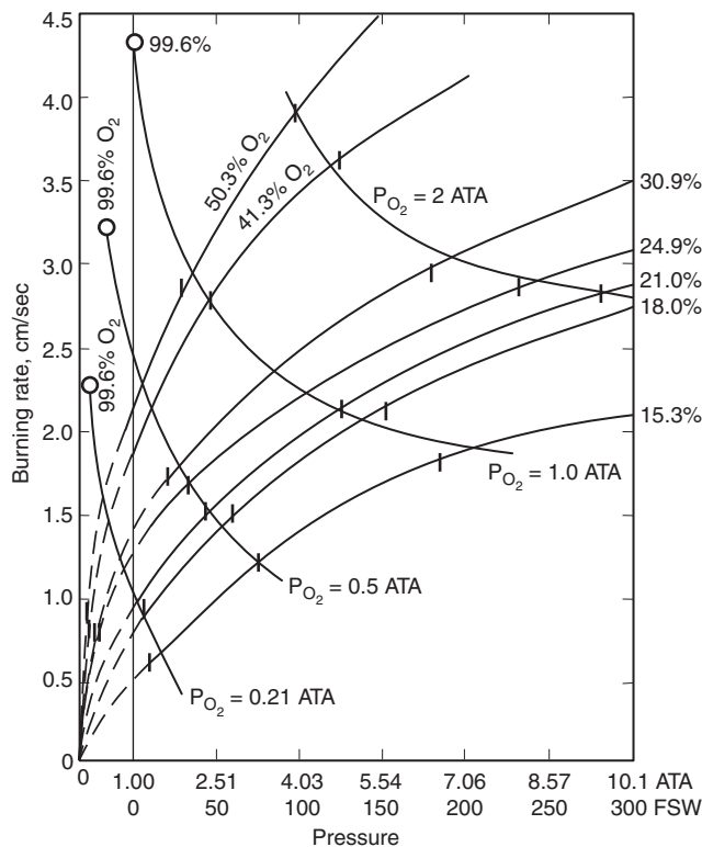
FIGURE A.3.3.2.3 Burning Rates of Filter Paper Strips at an Angle of 45 Degrees in N 2 -O 2 Mixtures. (Adapted from Figure 4 of “Technical Memorandum UCRI-721, Chamber Fire Safety.”)
