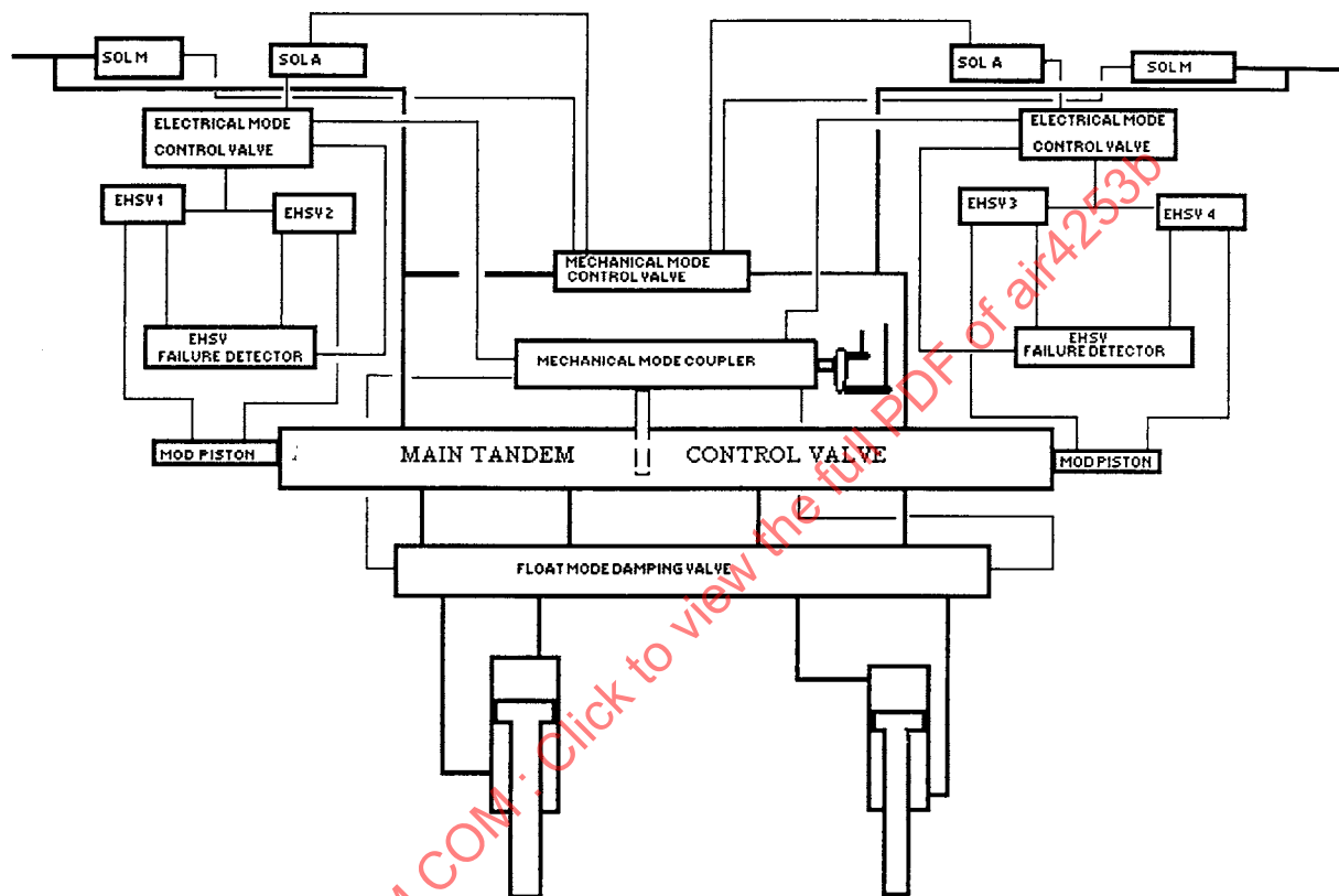
FIGURE 46 - C-17 PRIMARY FLIGHT CONTROL ACTUATION
