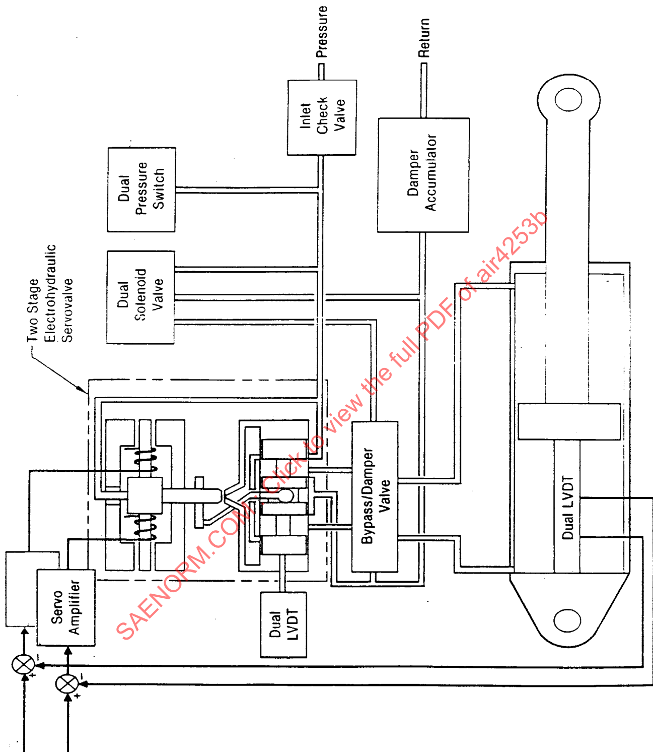
FIGURE 12 - F/A-18 A/B/C/D AILERON ACTUATOR SCHEMATIC
