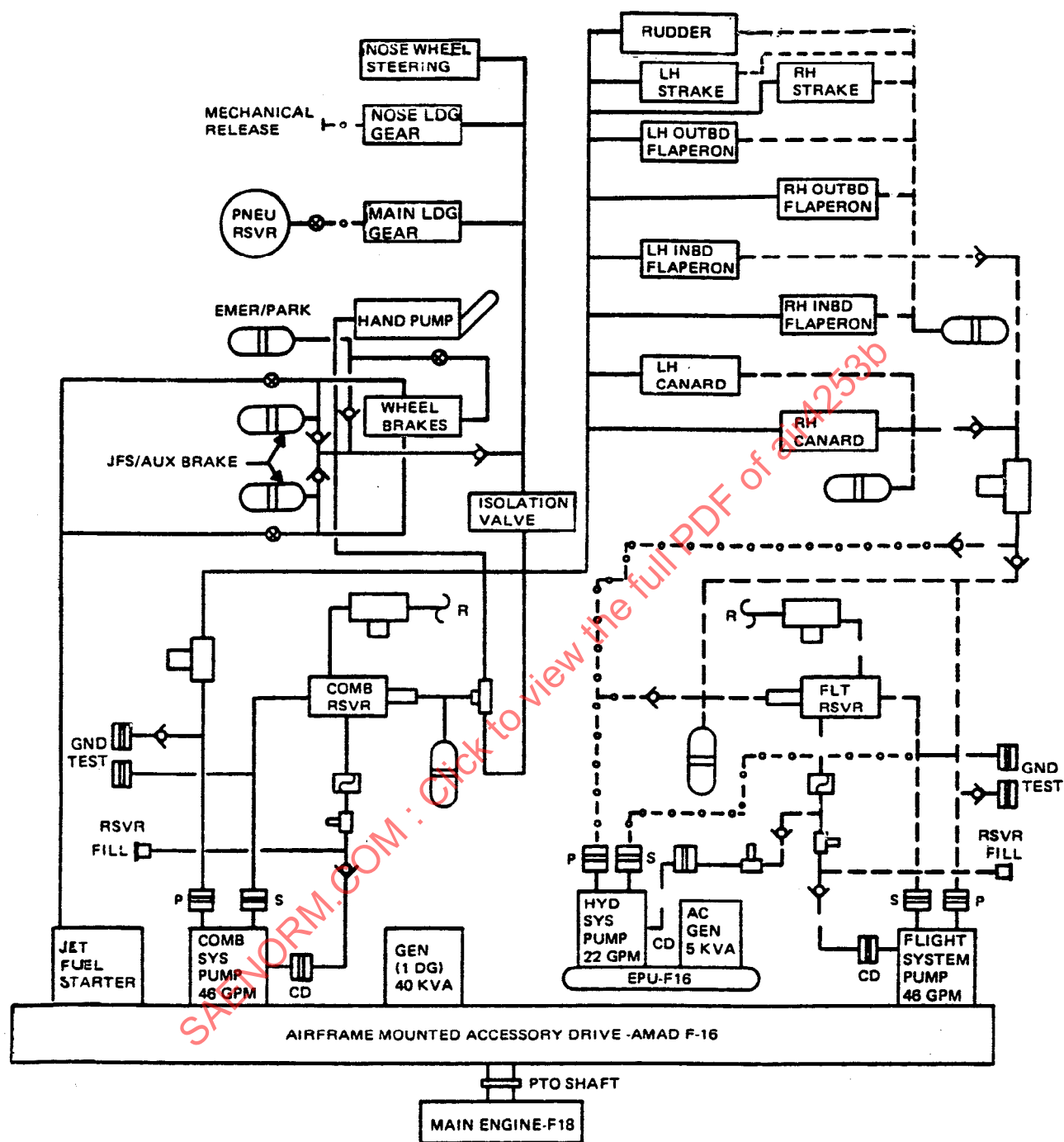
FIGURE 57 - X-29A FLIGHT CONTROL SYSTEM HYDRAULIC SCHEMATIC
