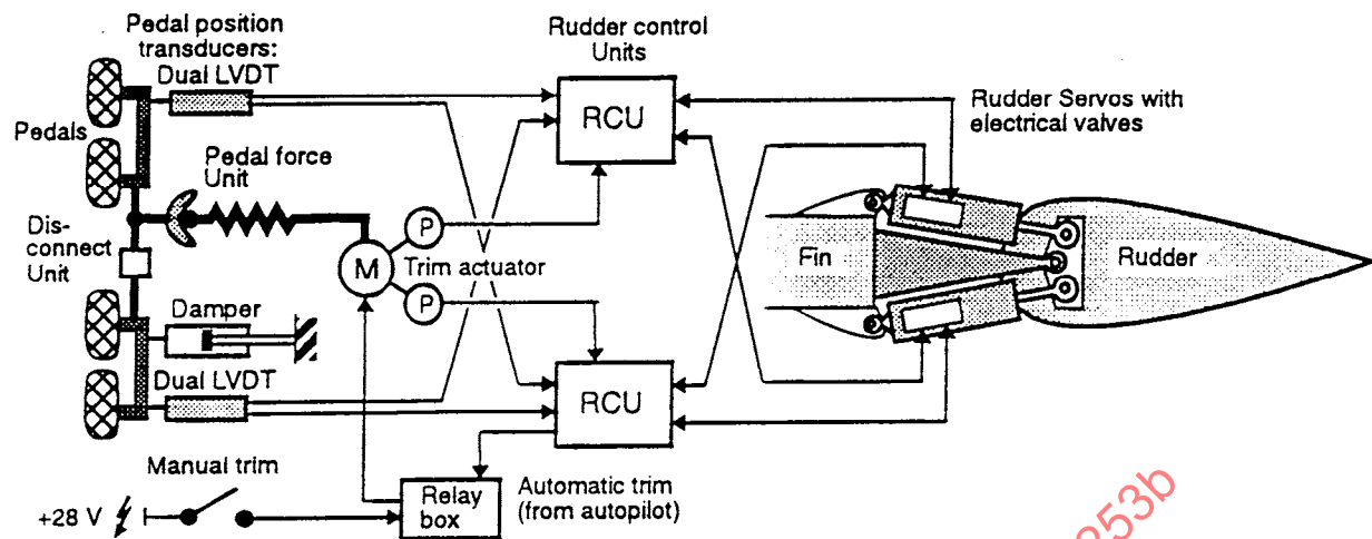
FIGURE 39 - SAAB 2000 RUDDER CONTROL SYSTEM FUNCTIONAL SCHEMATIC
