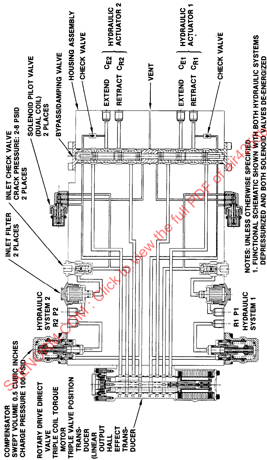
FIGURE 52 - X-31A RUDDER/CANARD CONTROL MODULE HYDRAULIC SCHEMATIC
