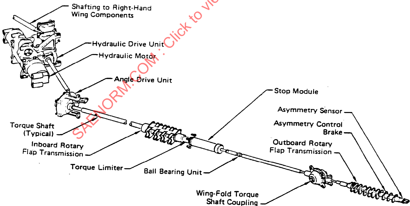
FIGURE 13 - F/A-18 A/B/C/D LEADING EDGE FLAP DRIVE SYSTEM
