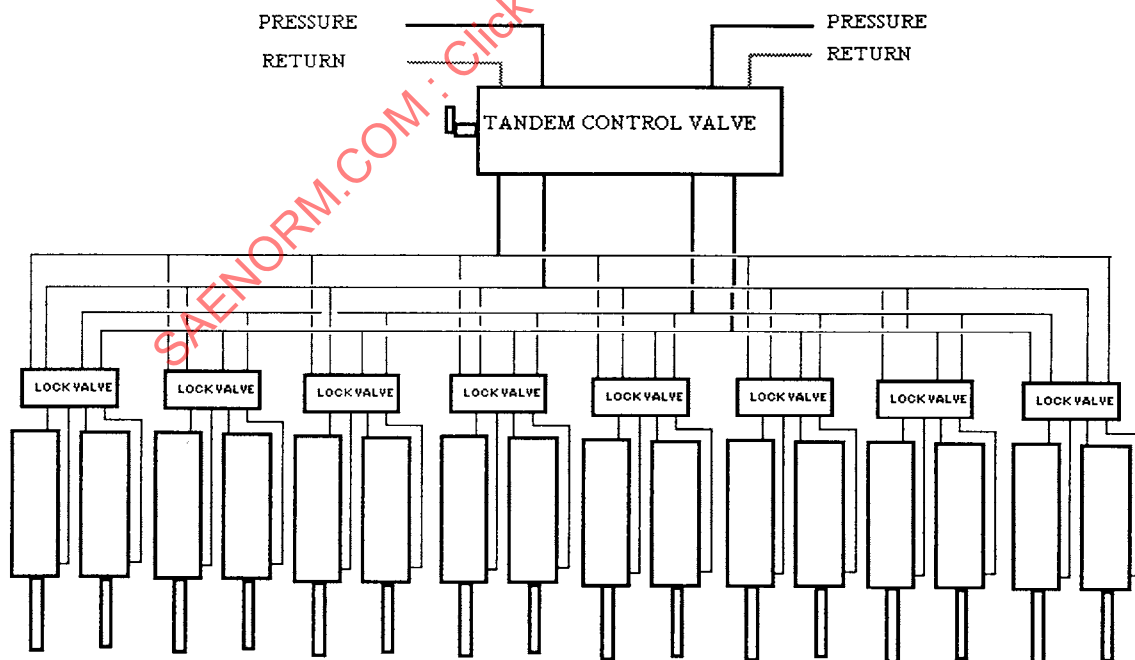
FIGURE 49 - C-17 SLAT ACTUATION
