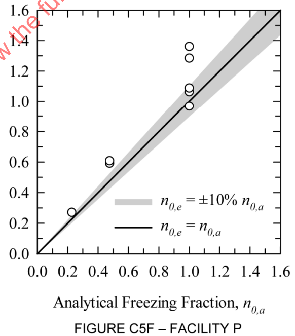
FIGURE C5 - FREEZING-FRACTION ANALYSIS FOR 36-IN-CHORD NACA 0012 AIRFOIL AT 3 DEGREES AOA CENTERLINE ICE SHAPES
