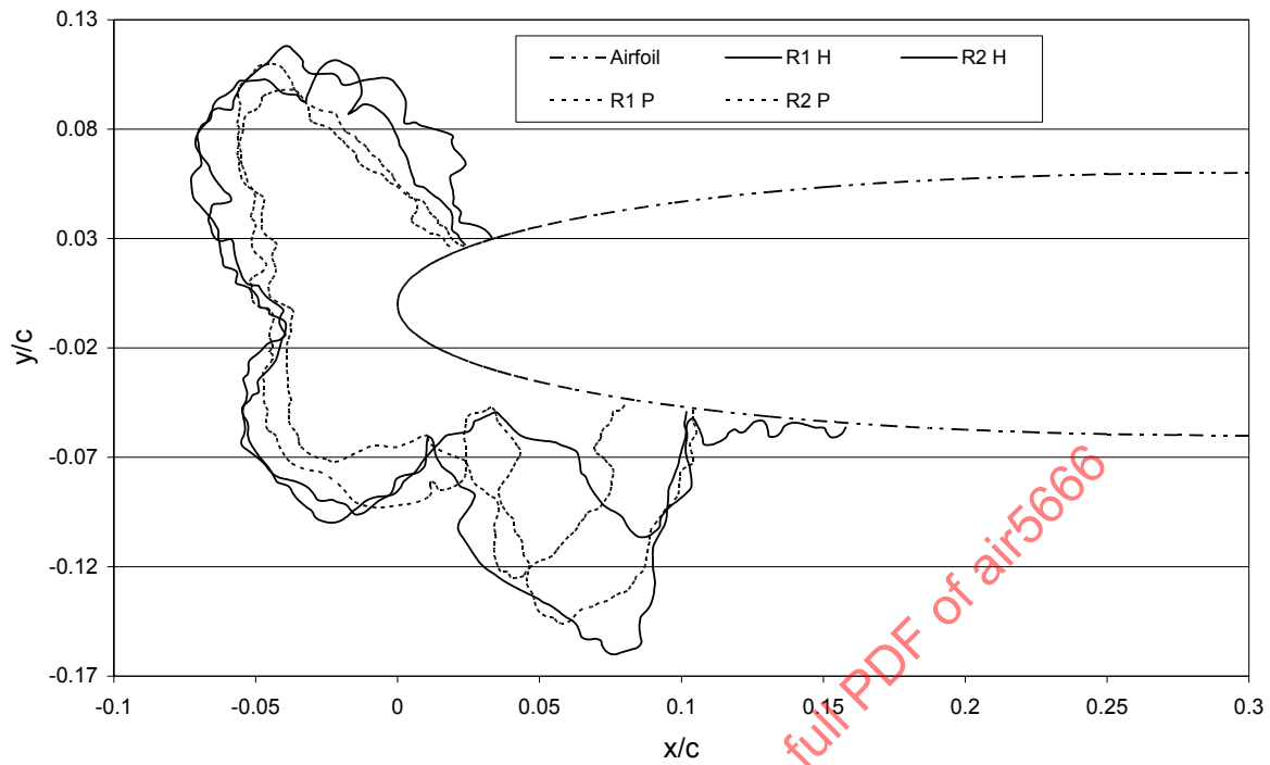
FIGURE D4C - TRACINGS FOR FACILITIES H AND P
