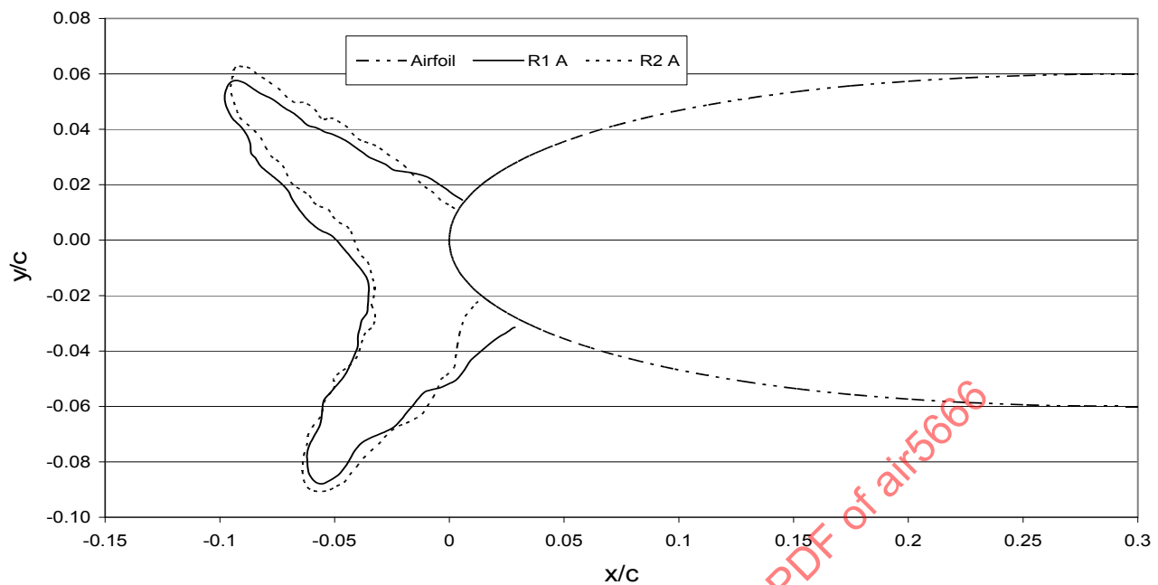
FIGURE 7 - ILLUSTRATION OF TYPICAL REPEATABILITY - FACILITY A CENTERLINE TRACINGS FOR CASE N12-02
