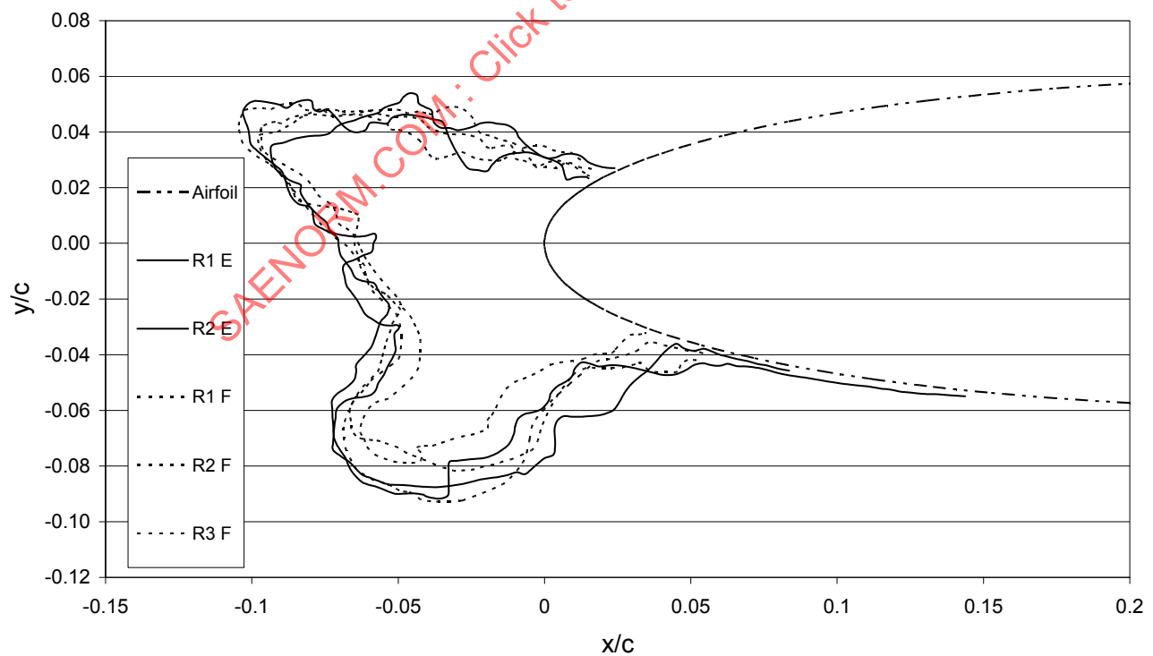
FIGURE D1C - TRACINGS FROM FACILITIES E AND F
