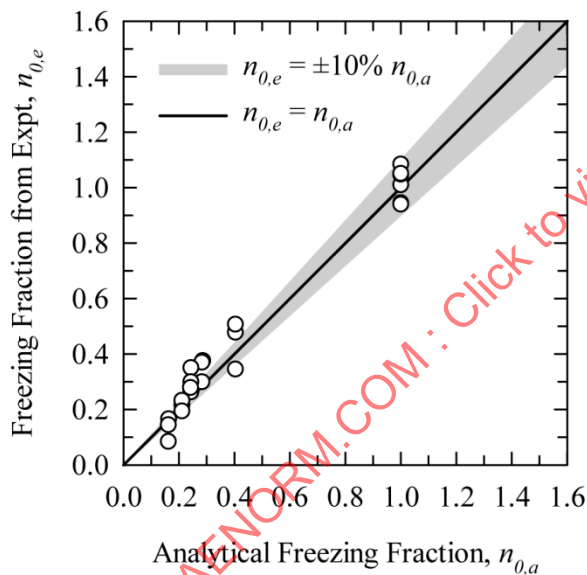
FIGURE C3 - FREEZING-FRACTION ANALYSIS RESULTS FOR CYLINDERS CENTERLINE ICE SHAPES
