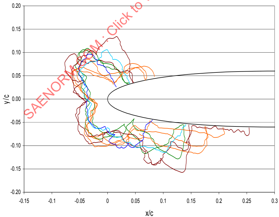
FIGURE 2 - CENTERLINE TRACINGS FROM ALL PARTICIPATING FACILITIES FOR THE 12 IN NACA 0012 AIRFOIL, TEST CONDITION 6 OF TABLE 2
