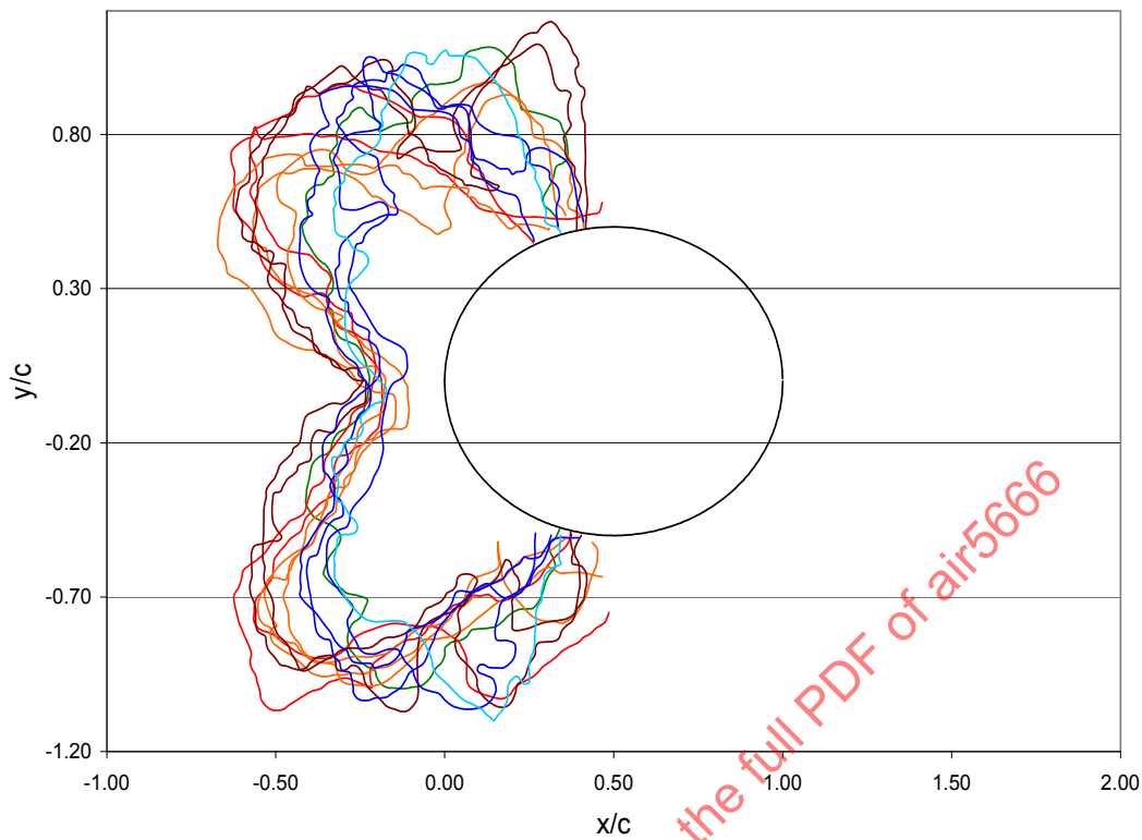
FIGURE 13 - CENTERLINE TRACINGS FROM ALL PARTICIPATING FACILITIES FOR THE 1.5 IN CYLINDER-FOR TEST CONDITION 6 OF TABLE 2
