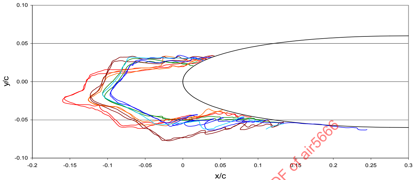
FIGURE 11 - CENTERLINE TRACINGS FROM ALL PARTICIPATING FACILITIES FOR THE 12 IN NACA 0012 AIRFOIL FOR TEST CONDITION 9 OF TABLE 2
