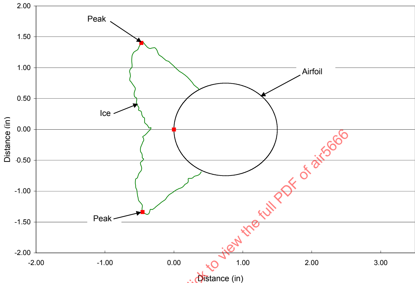
FIGURE B1 - EXAMPLE OF WRAPPED PLOT
