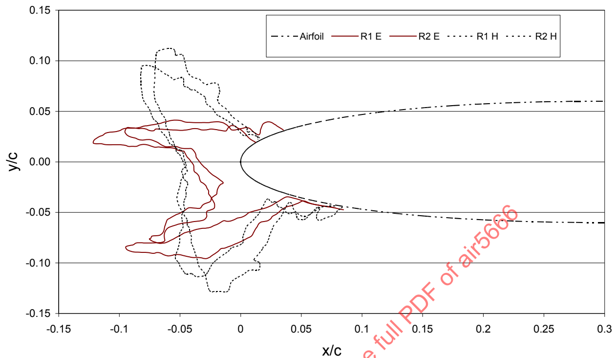
FIGURE D2C - TRACINGS FROM FACILITIES E AND H
