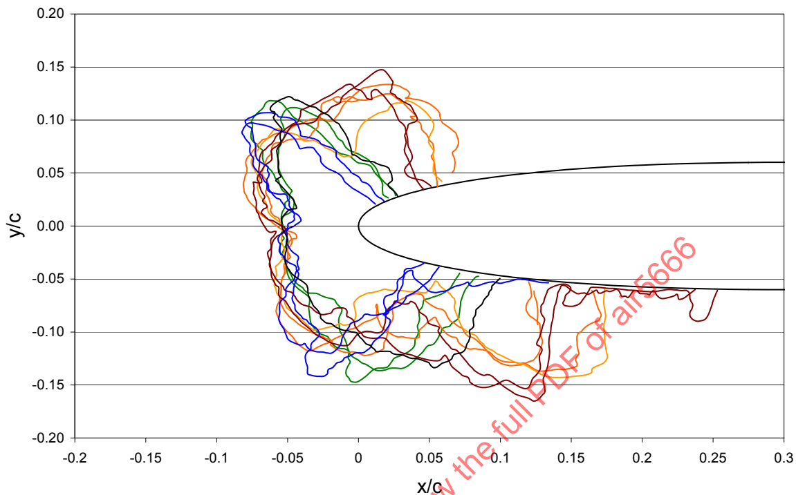
FIGURE D5A - TRACINGS FOR ALL FACILITIES
