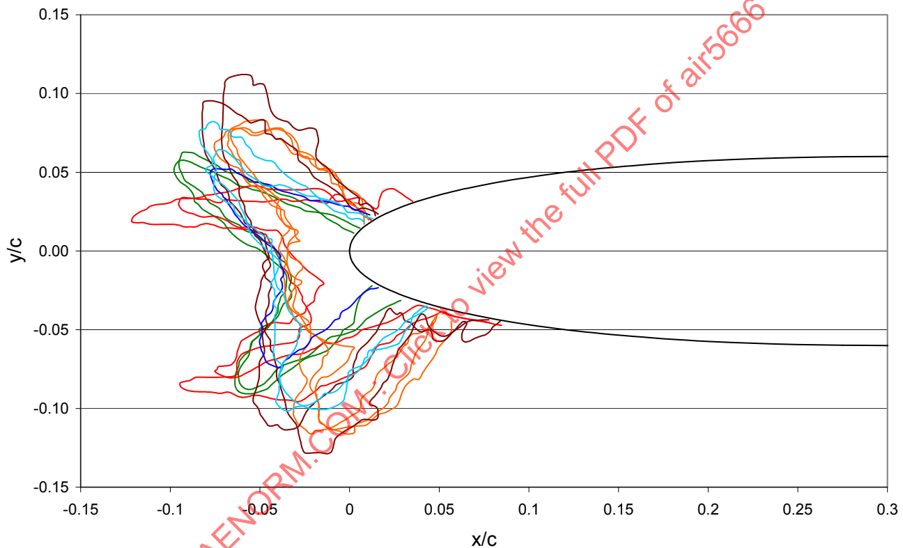
FIGURE 9 - CENTERLINE TRACINGS FROM ALL PARTICIPATING FACILITIES FOR THE 12 IN NACA 0012 AIRFOIL FOR TEST CONDITION 2 OF TABLE 2
