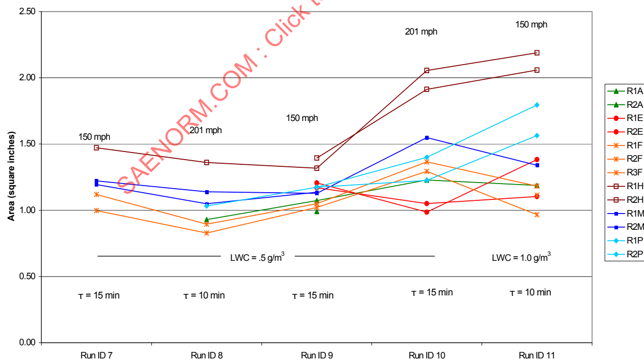
FIGURE 10D - 1.5 IN CYLINDER, RIME CASES (I.E., CASES 7 TO 11 OF TABLE 2)
