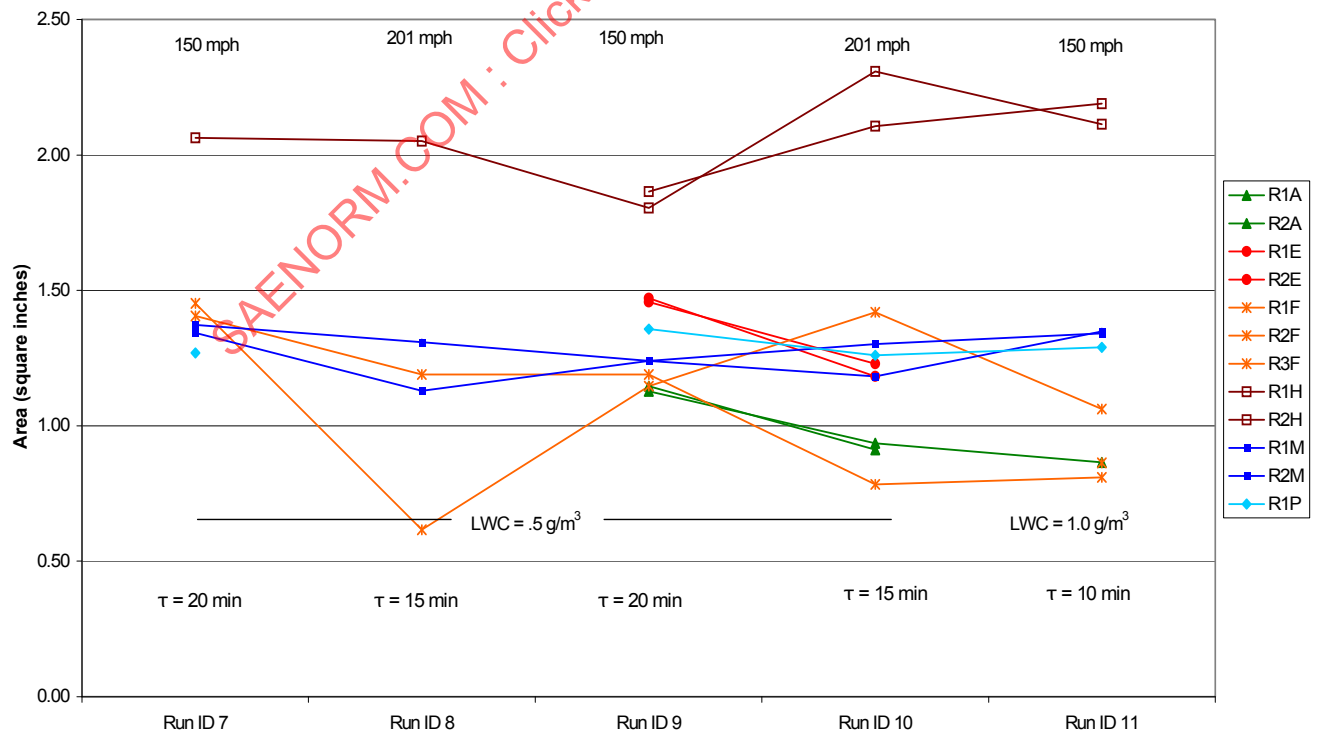
FIGURE 10B - 12 IN NACA 0012, RIME CASES (I.E., CASES 7 TO 11 OF TABLE 2)
