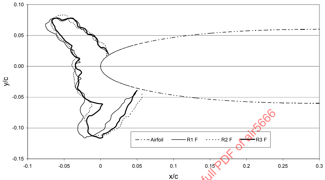
FIGURE 5 - ILLUSTRATION OF TYPICAL REPEATABILITY - FACILITY F CENTERLINE TRACINGS FOR CASE N12-02
