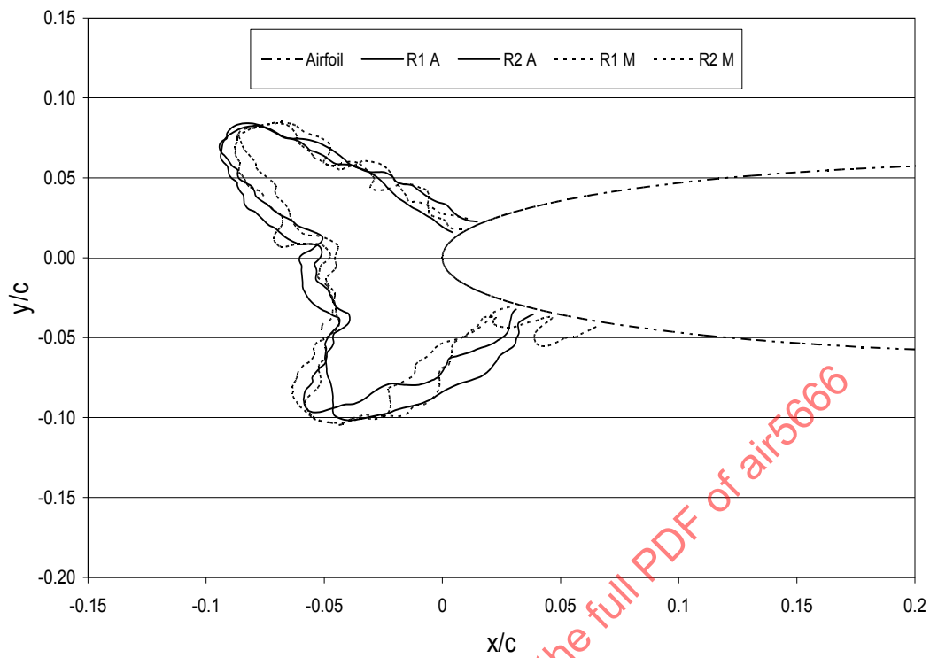
FIGURE D3B - TRACINGS FOR FACILITIES A AND M
