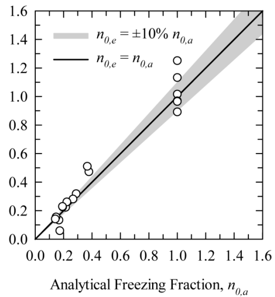
FIGURE C3B - FACILITY E
