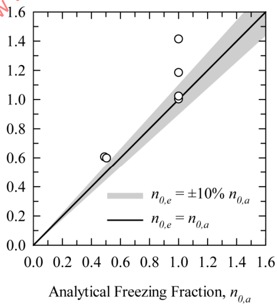
FIGURE C5B – FACILITY E
