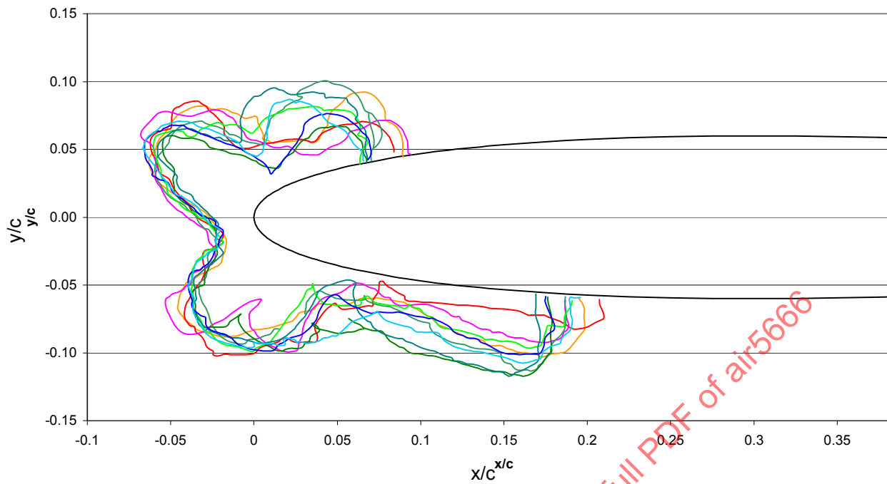
FIGURE 1 - SAMPLE PLOT OF ALL TRACINGS OBTAINED BY ONE OF THE PARTICIPATING FACILITIES FOR THE 12 IN NACA 0012 AIRFOIL, TEST CONDITION 6 OF TABLE 2
