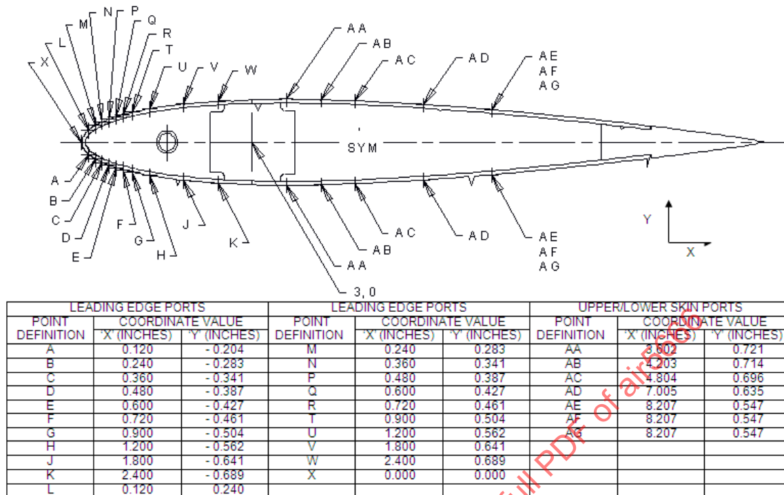
FIGURE A2 - 12 IN MODEL CROSS SECTION - PRESSURE TAP LOCATIONS
