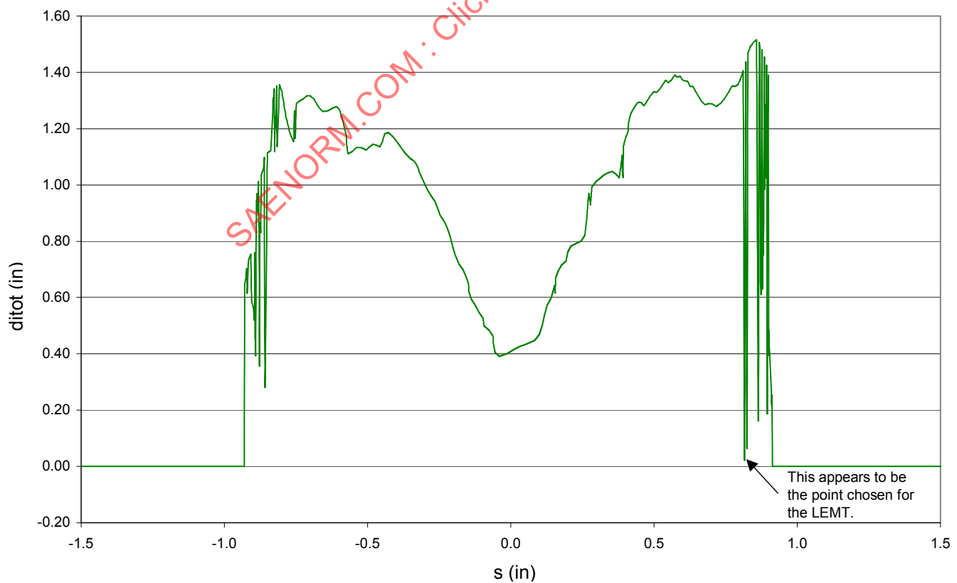
FIGURE B3 - EXAMPLE OF UNWRAPPED PLOT WITH ANOMALIES
