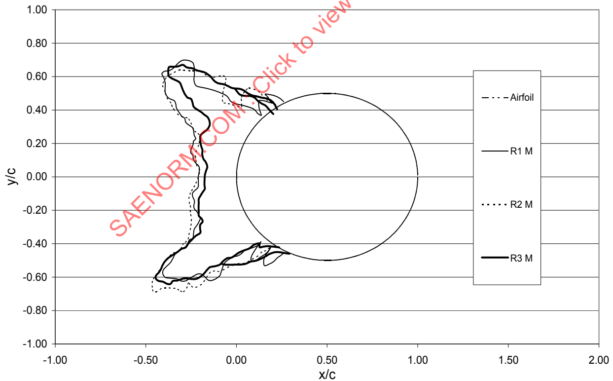
FIGURE 8 - ILLUSTRATION OF TYPICAL REPEATABILITY - FACILITY M CENTERLINE TRACINGS FOR CASE C15-02
