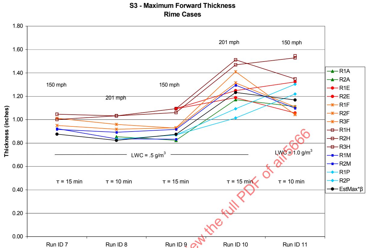
FIGURE B7 - S3 - RIME CASES
