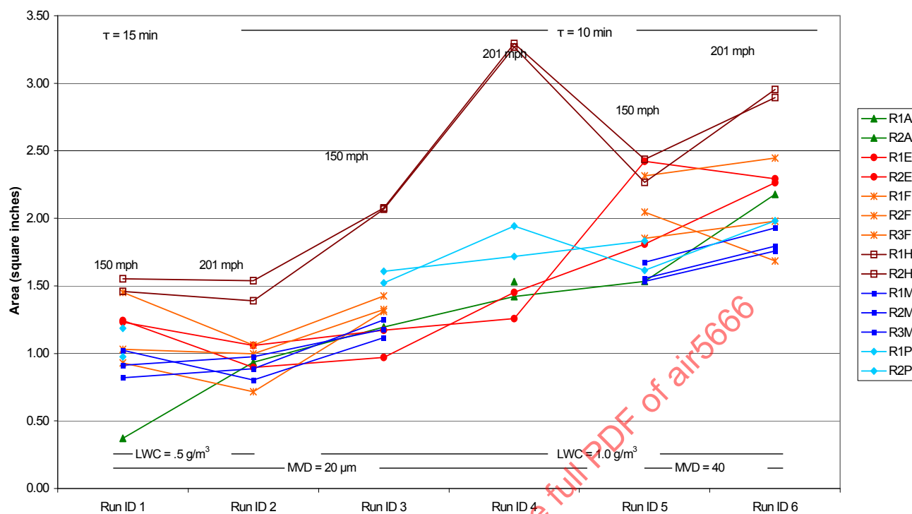
FIGURE 10C - 1.5 IN CYLINDER, GLAZE CASES (I.E., CASES 1 TO 6 OF TABLE 2)
