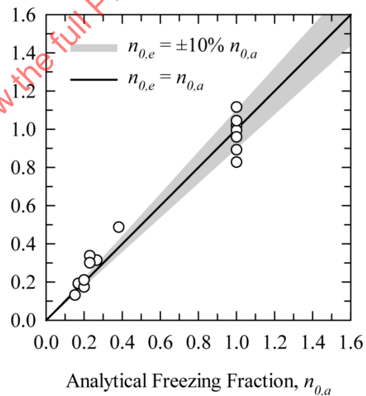
FIGURE C3 - FREEZING-FRACTION ANALYSIS RESULTS FOR CYLINDERS CENTERLINE ICE SHAPES
