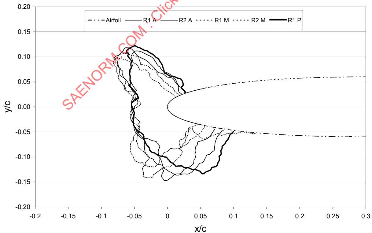
FIGURE D5B - TRACINGS FOR FACILITIES A, M AND P
