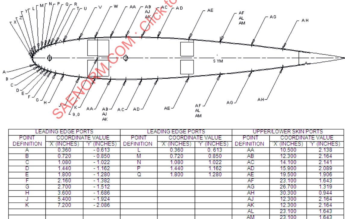
FIGURE A3 - 36 IN MODEL SECTION CUT - PRESSURE TAP LOCATIONS
