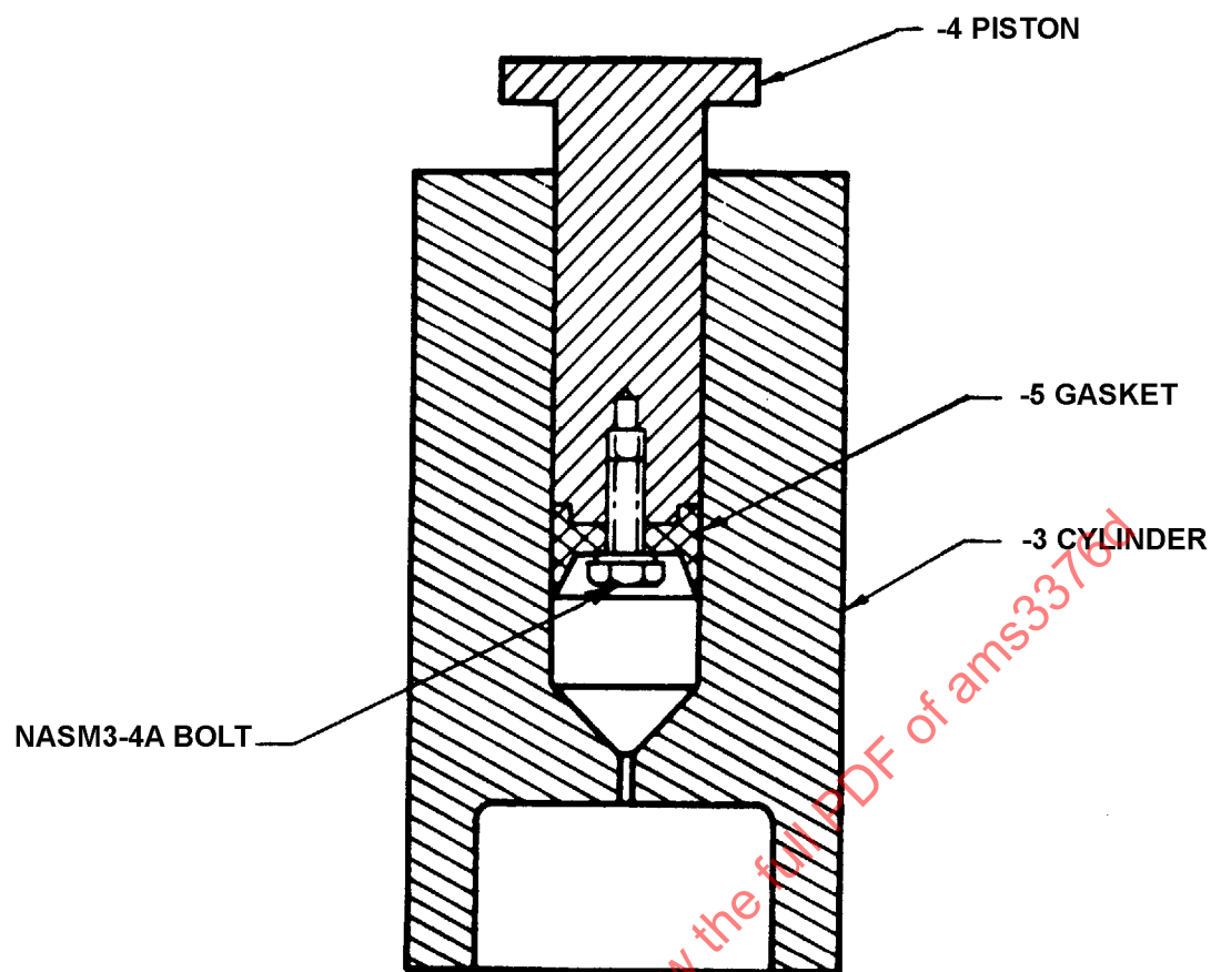
Figure 1 - Extrusion plastometer
