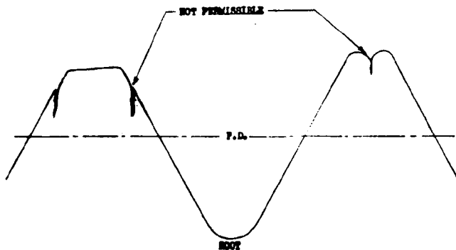
FIGURE 5 NOT PERMISSIBLE ROUND THREAD
