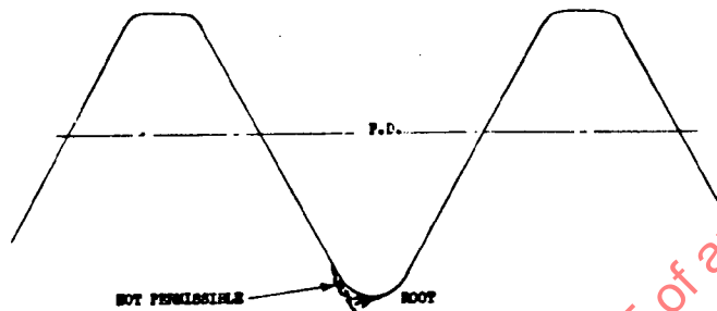
FIGURE 3 NOT PERMISSIBLE ROUND THREAD
