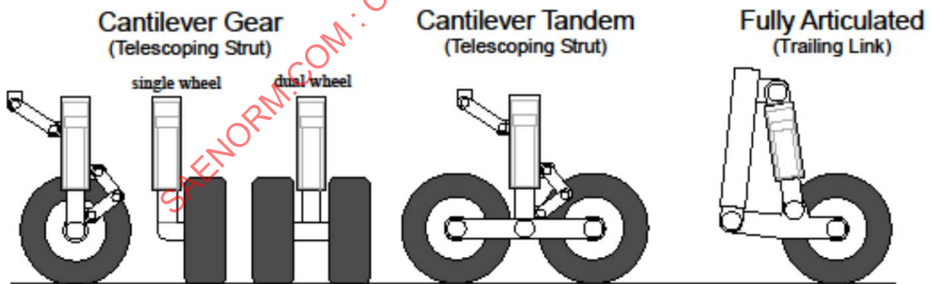
FIGURE 7 - TYPICAL TYPES OF MAIN GEAR
