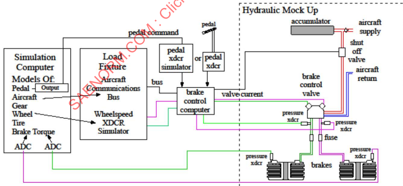
FIGURE 16 - HARDWARE IN THE LOOP EXAMPLE, BRAKE BY WIRE SYSTEM
