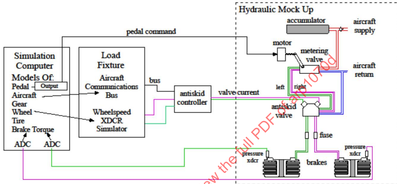
FIGURE 15 - HARDWARE IN THE LOOP EXAMPLE, ANTISKID SYSTEM
