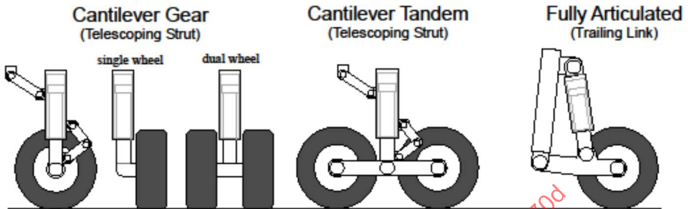
FIGURE 19 - TYPICAL TYPES OF MAIN GEAR
