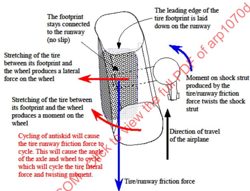
FIGURE 12 - TIRE TWIST
