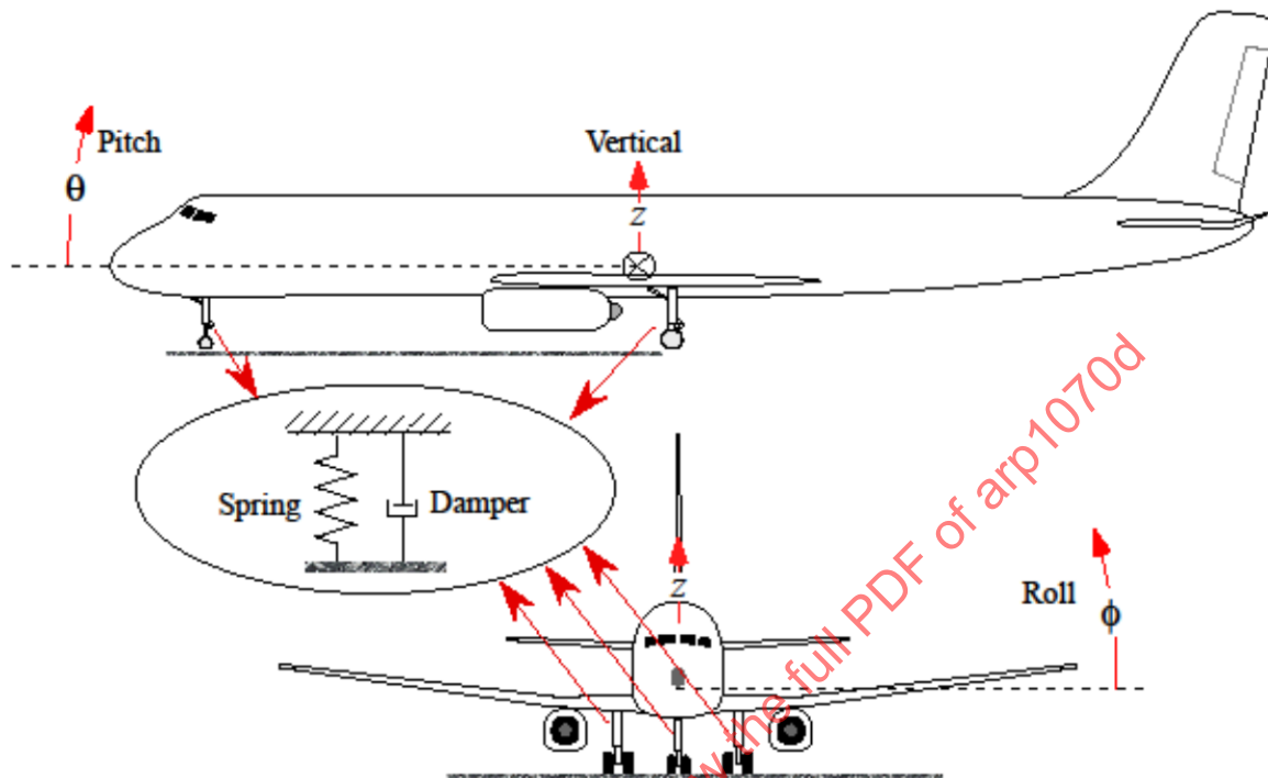
FIGURE 8 - SUSPENSION
