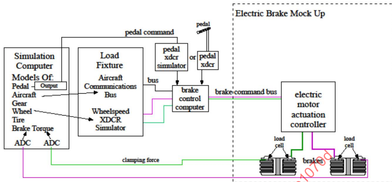
FIGURE 17 - HARDWARE IN THE LOOP EXAMPLE, ELECTRIC BRAKE SYSTEM
