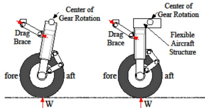
FIGURE 11 - FORWARD RAKED GEAR
