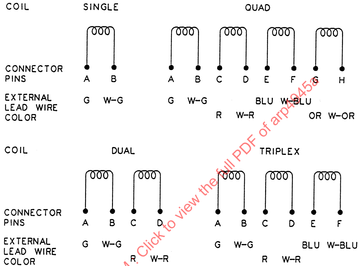
FIGURE 5 - Connector Pin Identification and Wire Color Coding
