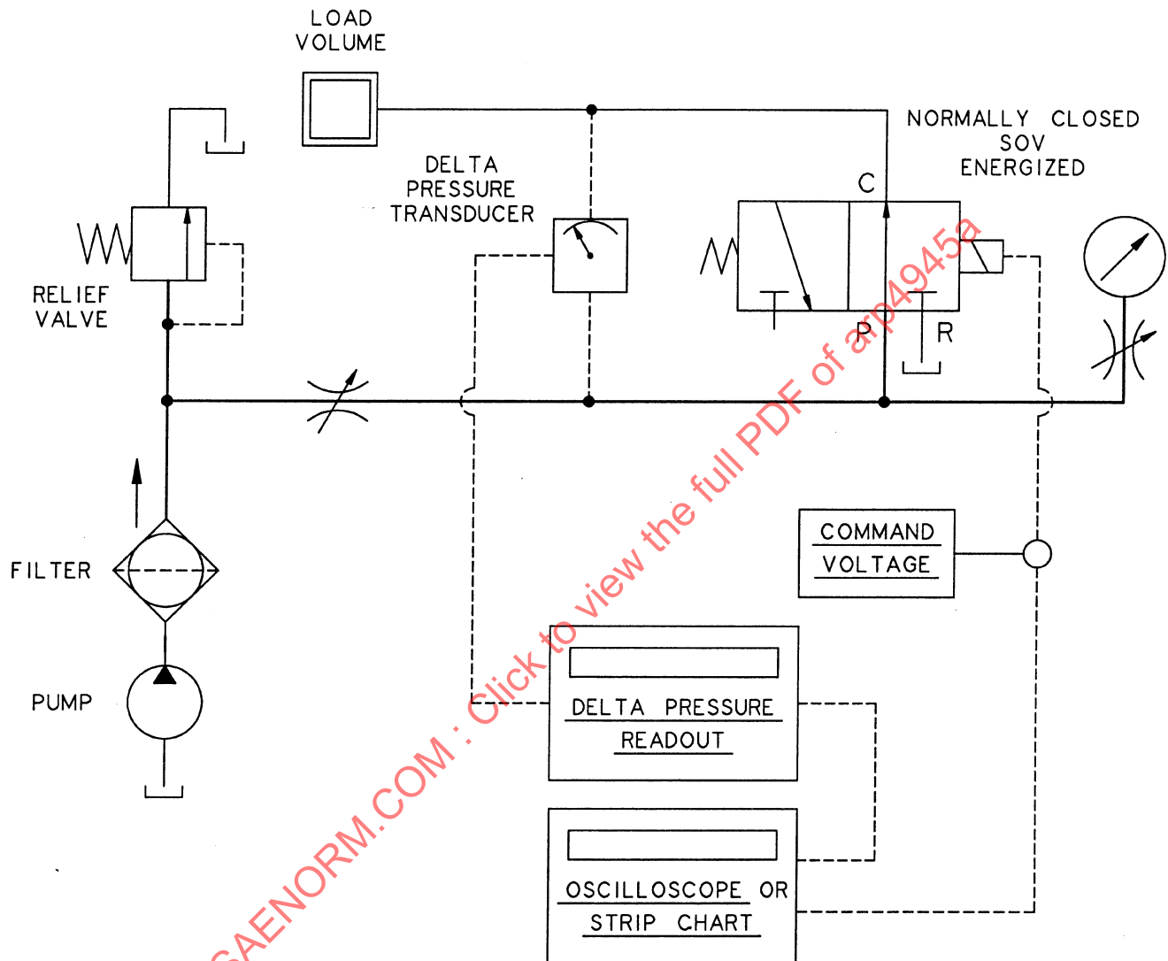
FIGURE 7 - Test Set-up for Response Time
