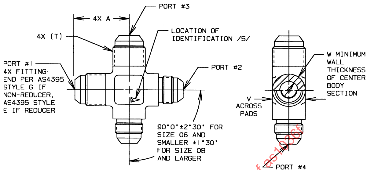
FIGURE 1 - CROSS, FLARED
