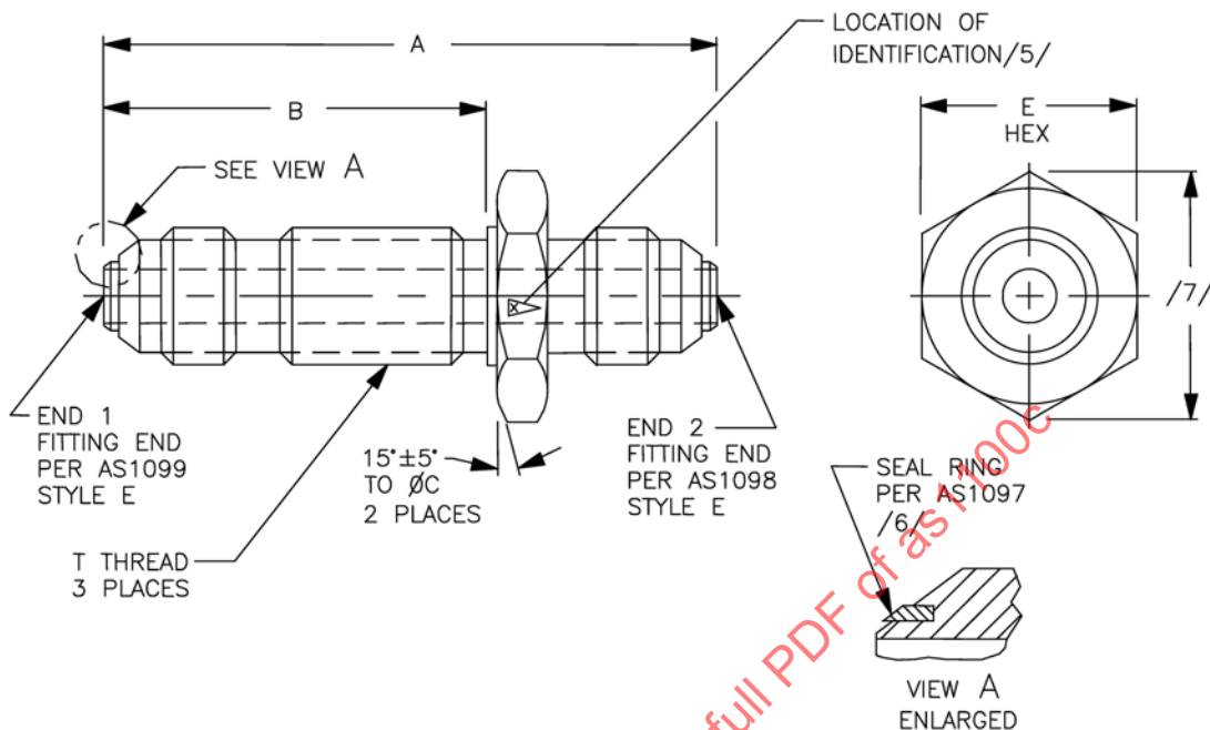
FIGURE 1 - FITTING, UNION, FLARED TUBE BULKHEAD AND UNIVERSAL
