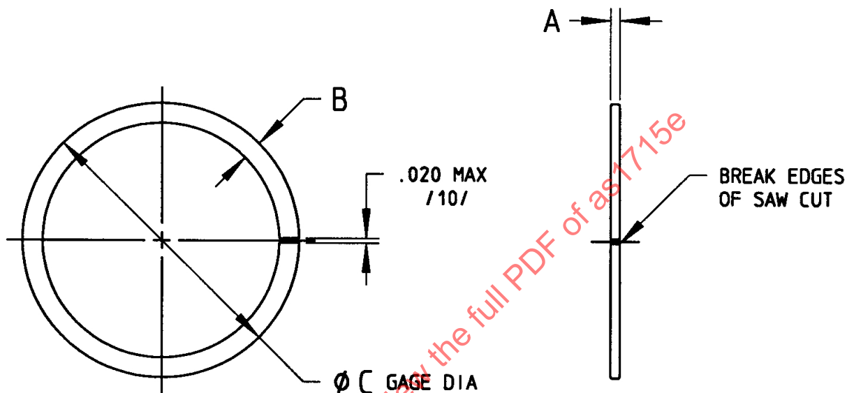
FIGURE 1 - WASHER
