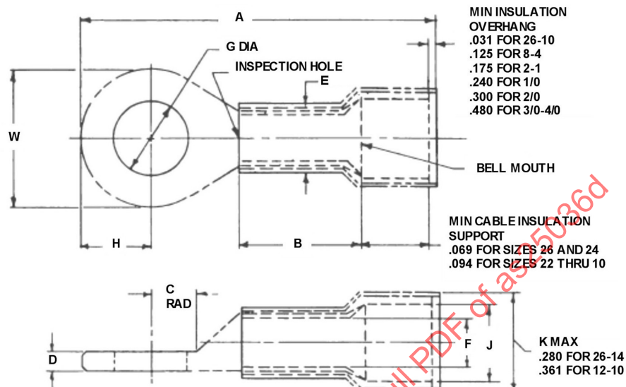
FIGURE 1 – TERMINAL CONSTRUCTION
