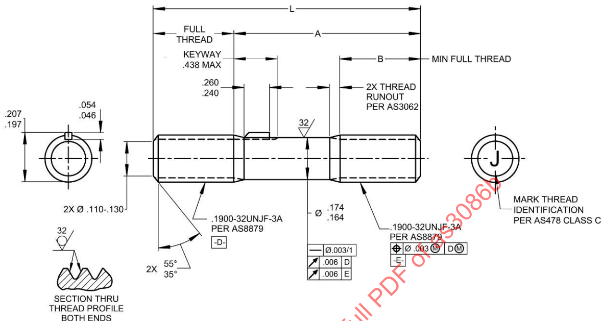
FIGURE 1 - STUD
