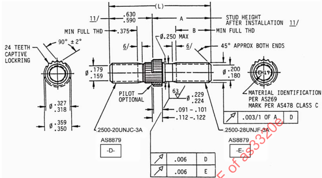
FIGURE 1 - STUD
