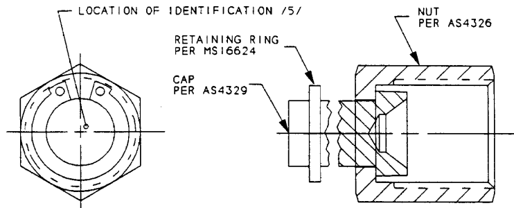
FIGURE 1 - CAP ASSEMBLY, BASIC
