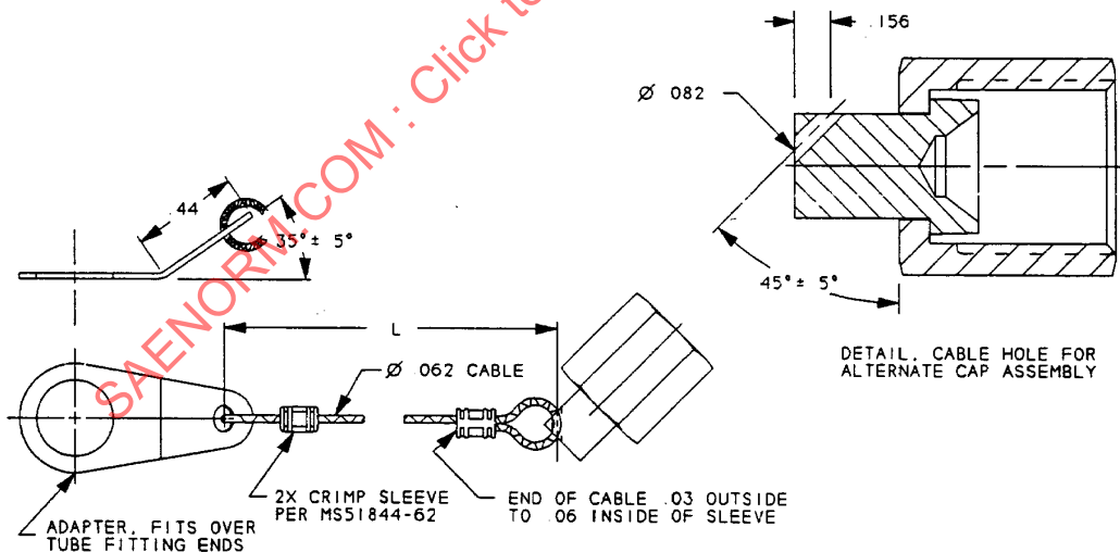
FIGURE 3 - ALTERNATE CAP ASSEMBLY
