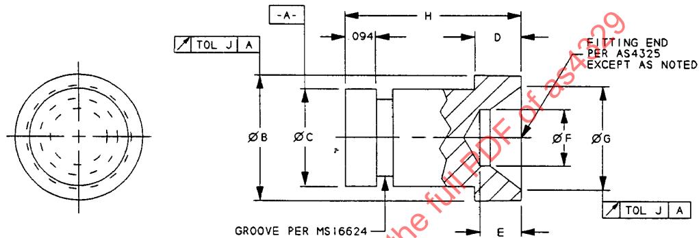
FIGURE 2 - CAP DETAIL
