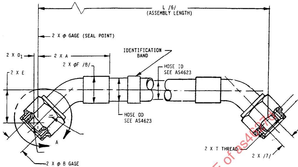
FIGURE 1 - HOSE ASSEMBLY, 45° ELBOW TO 45° ELBOW
