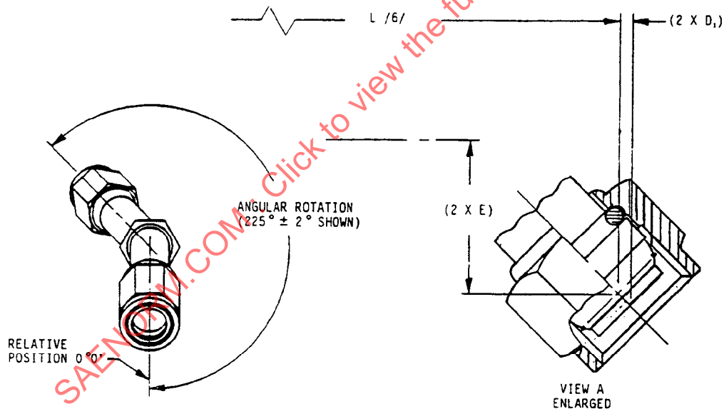
FIGURE 2 - FITTING ORIENTATION /19/
