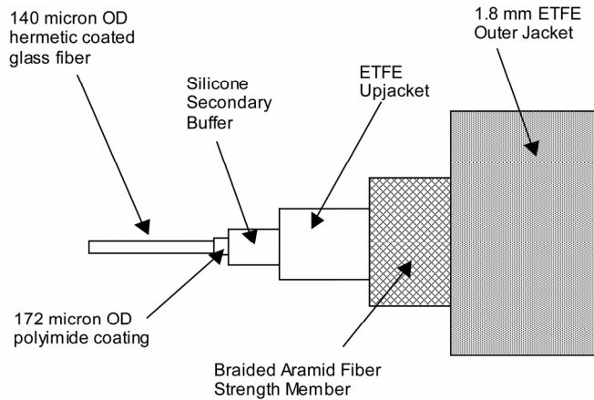
FIGURE 1 - CABLE CONFIGURATION
