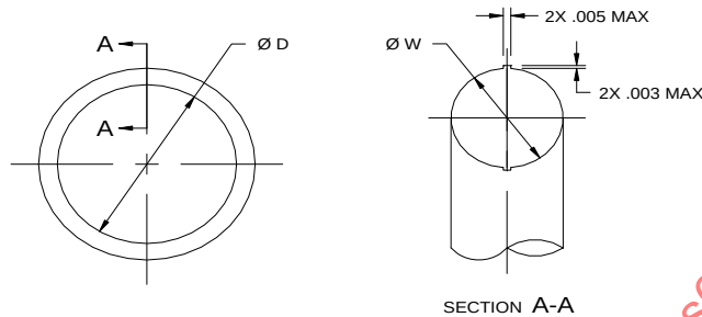
FIGURE 1 - BOSS O-RING DIMENSIONS FOR TABLE 1 WIDTH (ØW) AND INSIDE DIAMETER (ØD)
