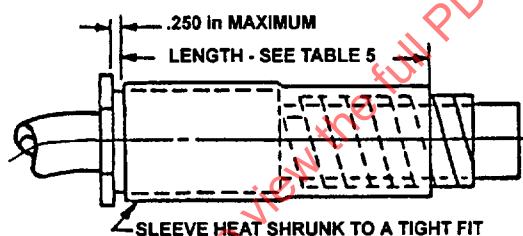
FIGURE 2 - TUBULAR/COIL ABRASION END /10/ /11/
