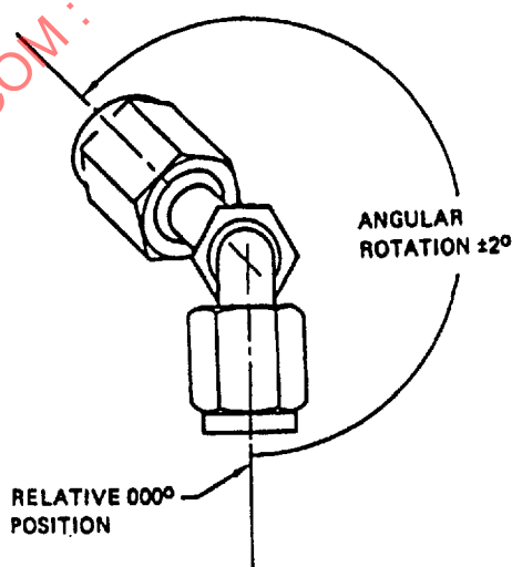
FIGURE 3 - FITTING ANGULAR ORIENTATION /19/
