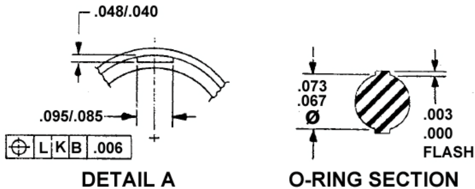
FIGURE 1A - DUMMY STOWAGE RECEPTACLE (DETAIL A)
