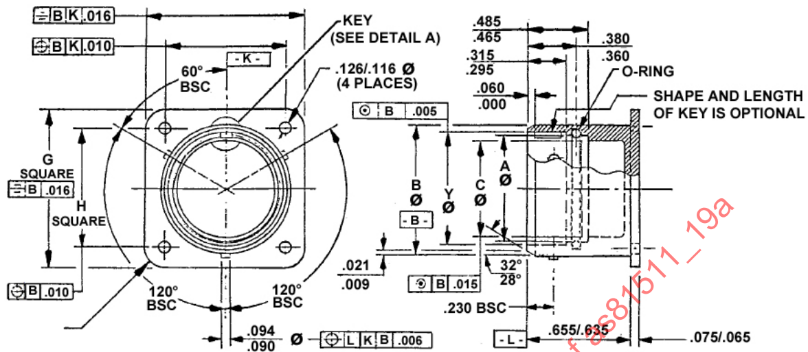
FIGURE 1 - DUMMY STOWAGE RECEPTACLE
