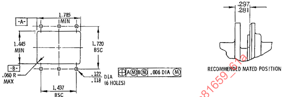
SUGGESTED PANEL CUT-OUT DIMENSIONS
