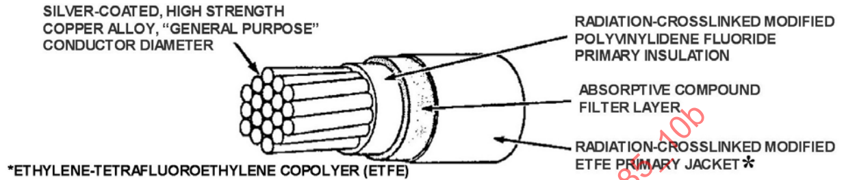
FIGURE 1 - AS85485/10 CONFIGURATION
