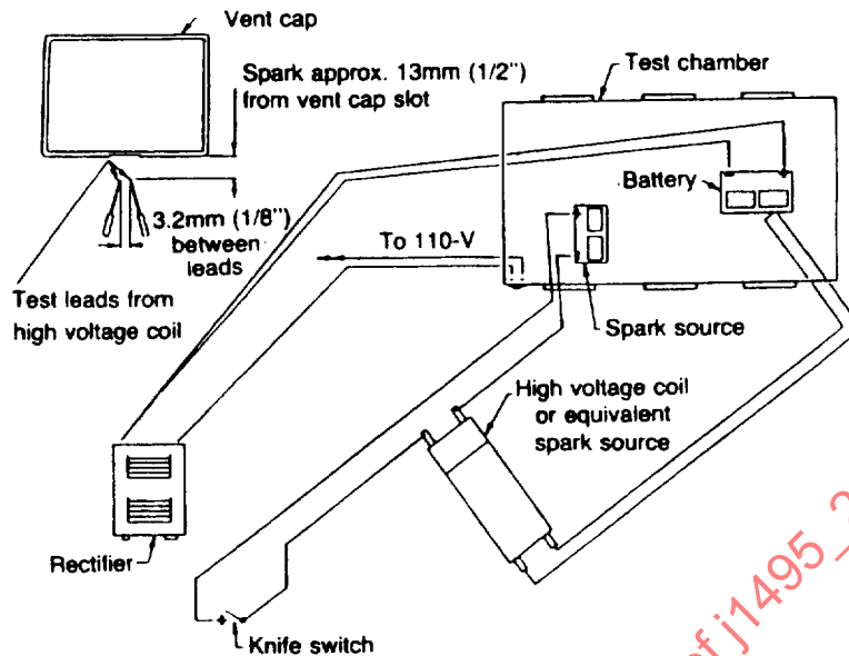
FIGURE 2A—SCHEMATIC FOR TEST ON BATTERY
