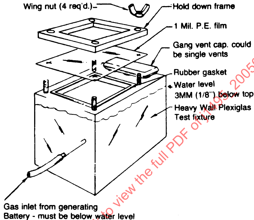
FIGURE 3—TEST FIXTURE
