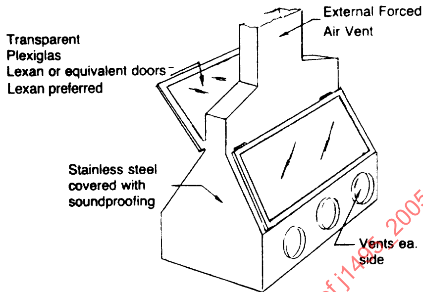
FIGURE 1—TEST CHAMBER
