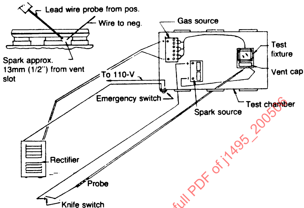
FIGURE 4—SCHEMATIC FOR TEXT FIXTURE
