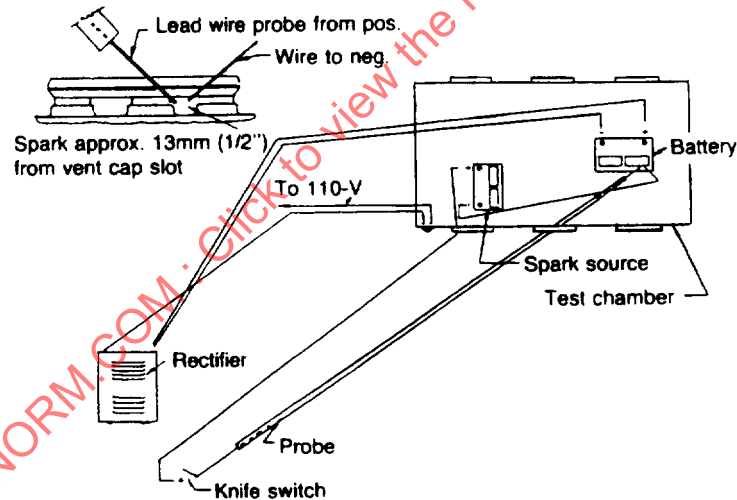
FIGURE 2B—SCHEMATIC FOR TEST ON BATTERY
