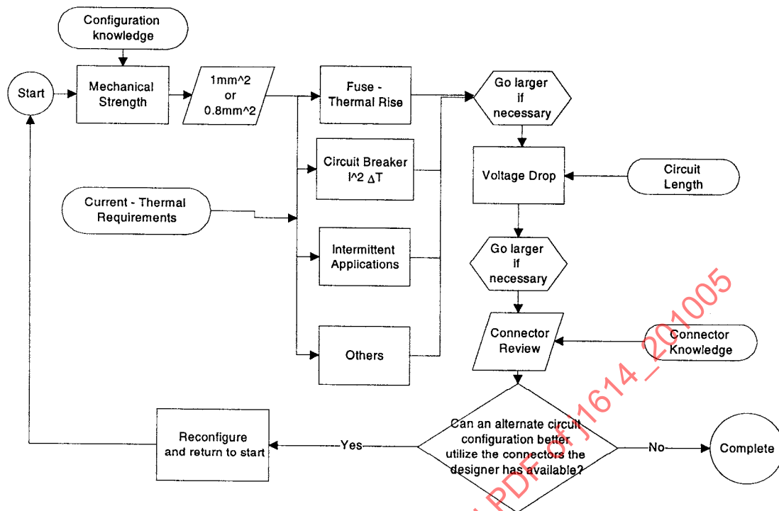
FIGURE 1 - CABLE SIZING FLOWCHART
