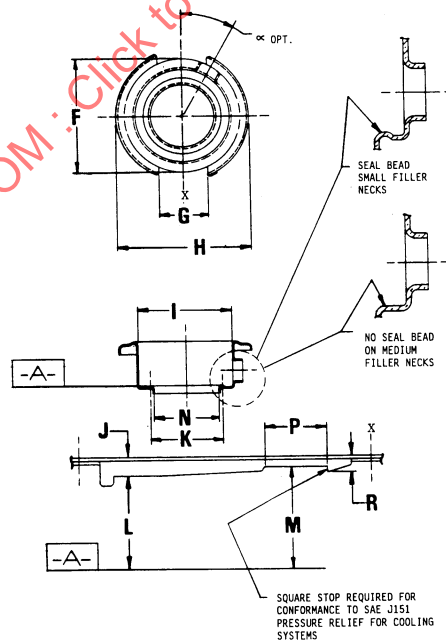
FIGURE 2—RADIATOR FILLER NECKS
