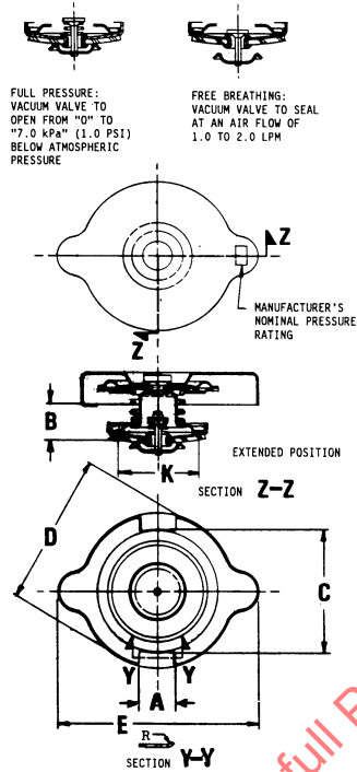
FIGURE 1—PRESSURE TYPE RADIATOR CAP
