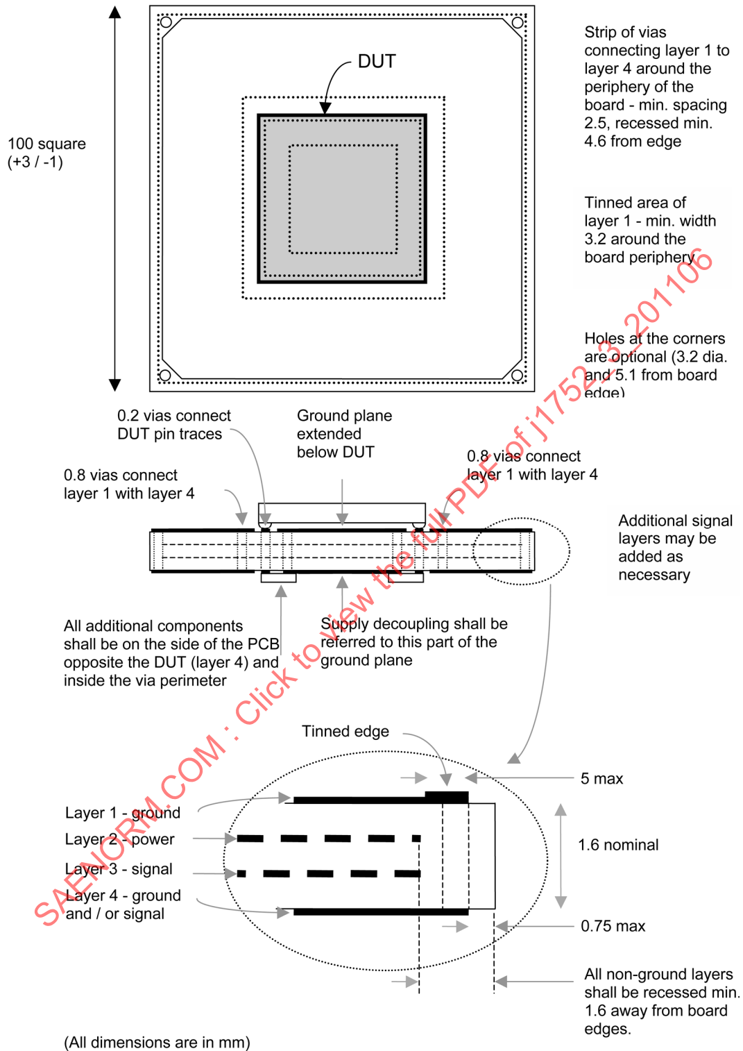
FIGURE 4 - IC TEST PRINTED CIRCUIT BOARD
