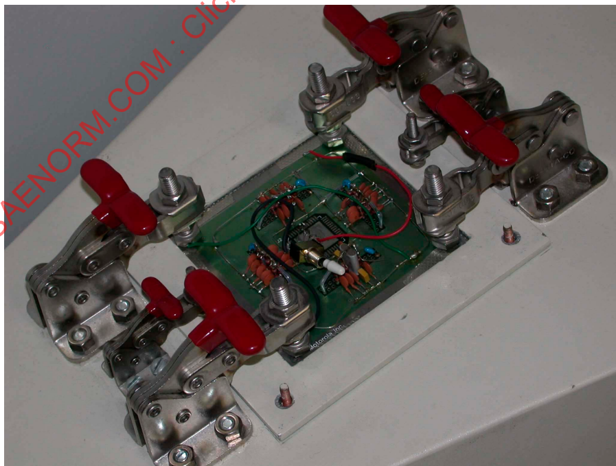
FIGURE 3 - WIDEBAND TEM CELL WITH DETAIL OF TEST PCB AND PORT
