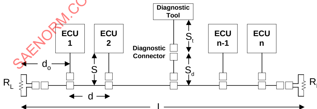
FIGURE 2 - WIRING NETWORK TOPOLOGY (TYPE I ECUS ONLY)
