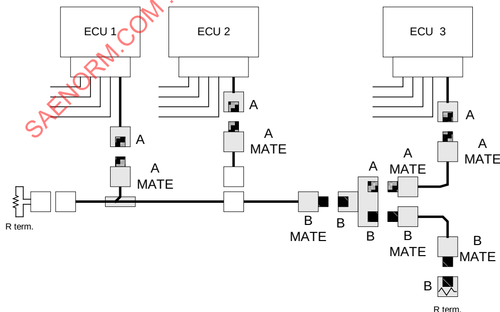
FIGURE 5 - AN EXAMPLE OF SAE J1939-11 CONNECTOR USAGE IN A SAE J1939-15 NETWORK
