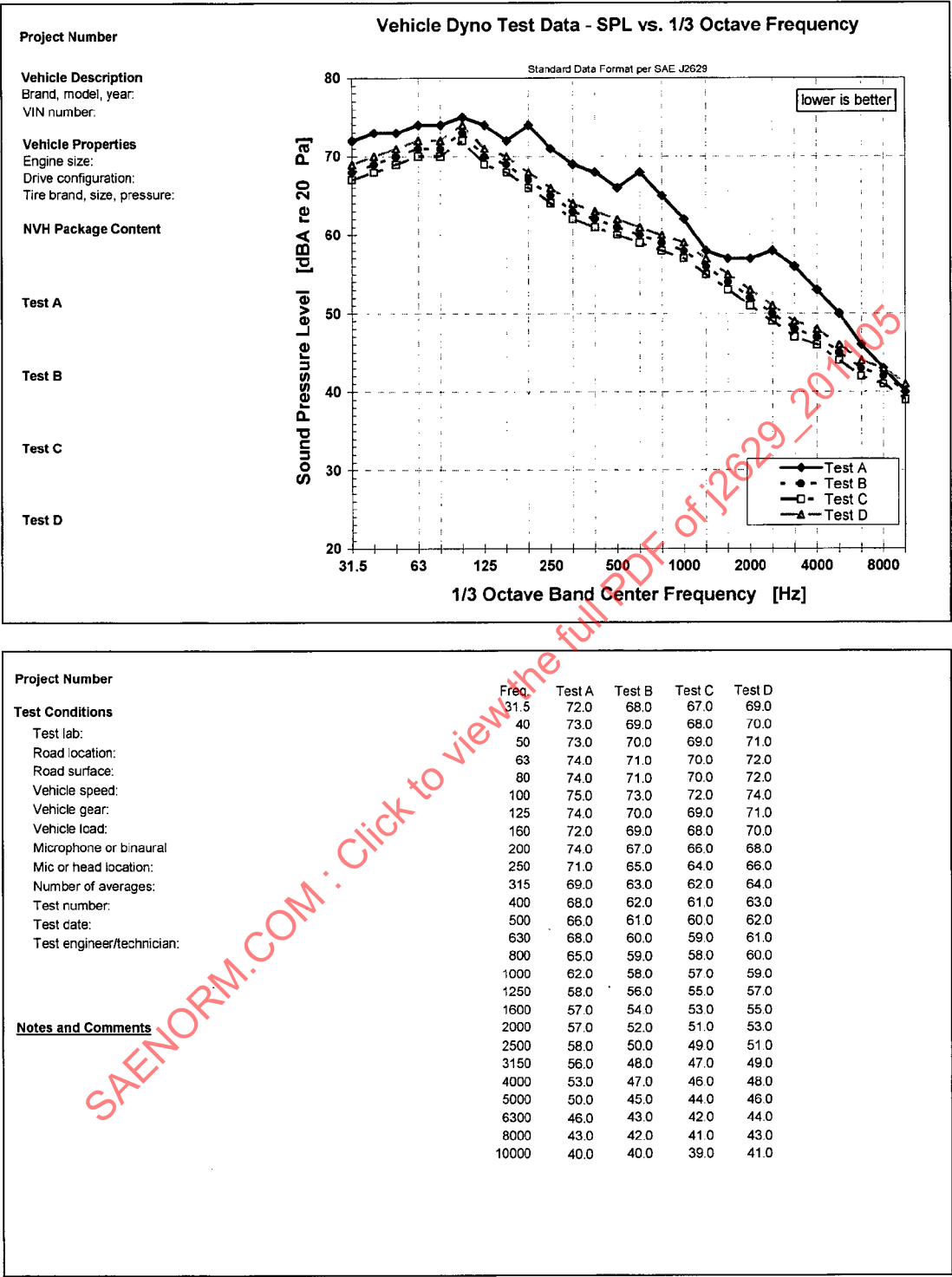
FIGURE 4 - VEHICLE DYNO DATA - A-WEIGHTED SOUND PRESSURE LEVEL VS. 1/3 OCTAVE FREQUENCY
