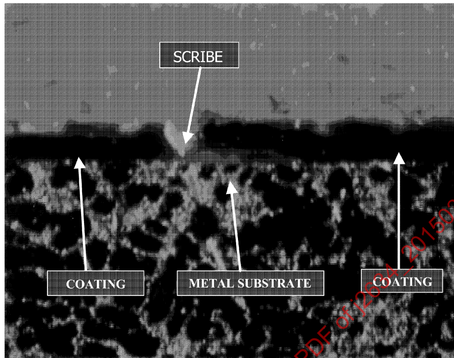
FIGURE 5—SCRIBED WITH INSUFFICIENT PRESSURE TO CUT THROUGH TO SUBSTRATE
