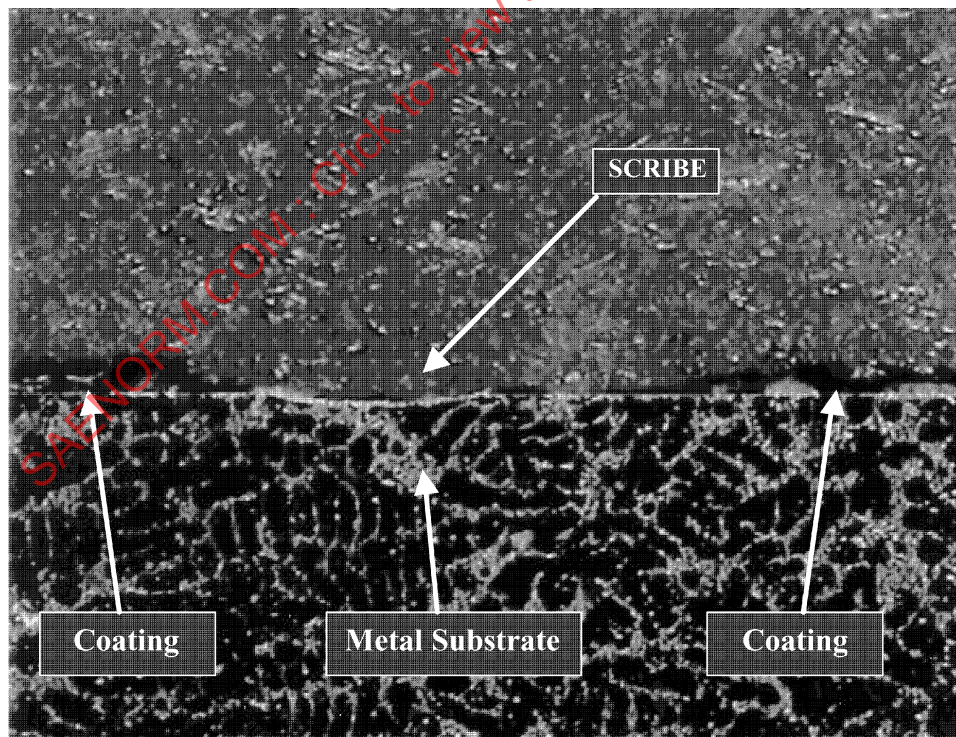
FIGURE 4—A BROKEN SCRIBE TOOL RESULTS IN NO V-NOTCH AND THE PAINT FILM IS REMOVED ON THE SURFACE
