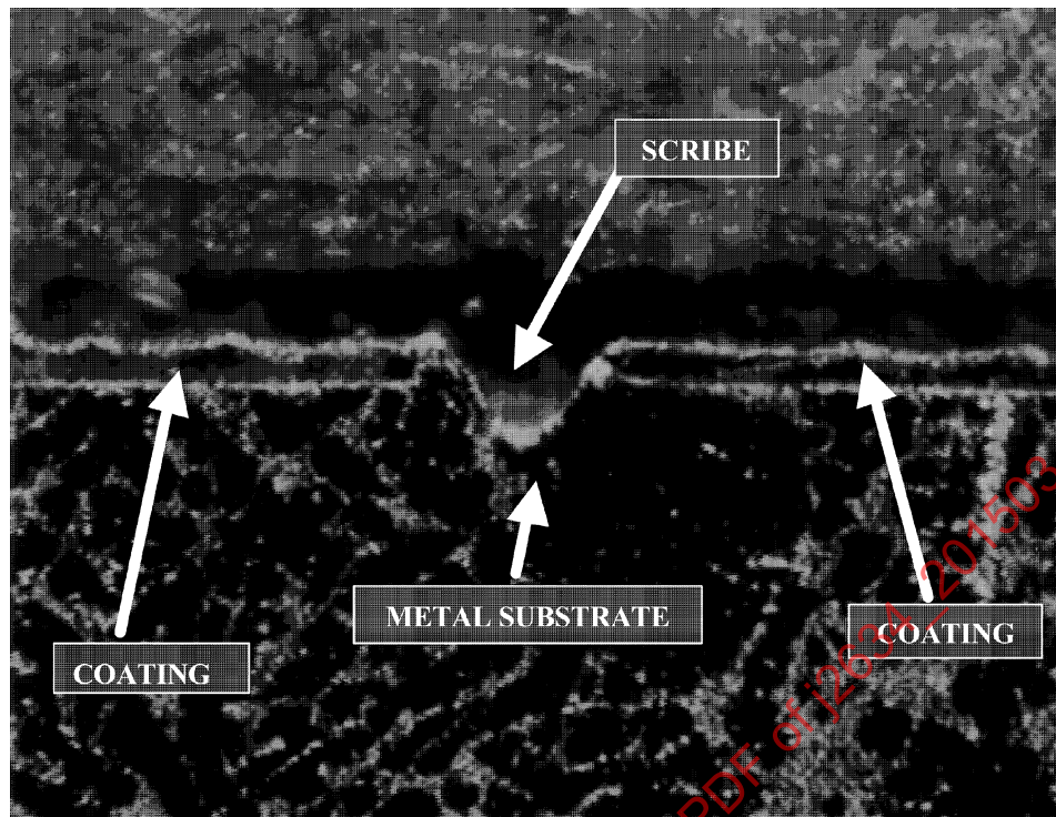
FIGURE 3—CORRECT SCRIBING, UNIFORM AND SYMMETRICAL SCRIBE
