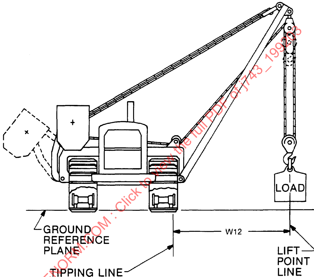
FIGURE 1—PIPELAYER
