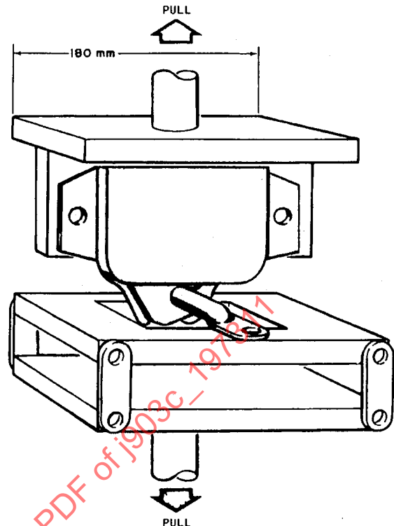
φ FIG. 2—SUGGESTED HOOD LATCH STATIC TEST FIXTURE
