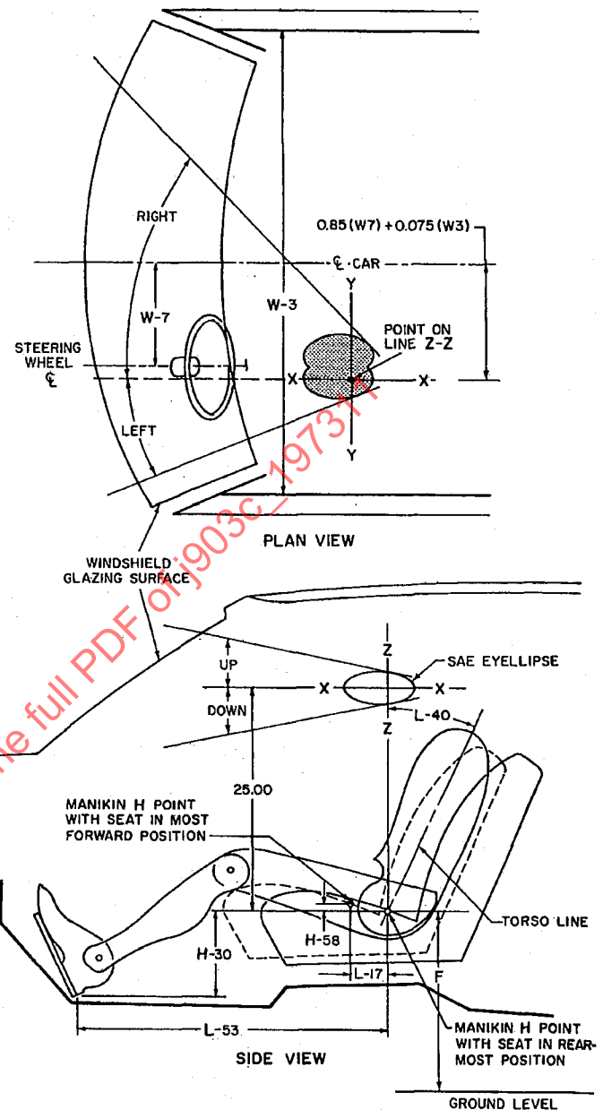
FIG. 1—EYELIPSE TEMPLATE LOCATION
