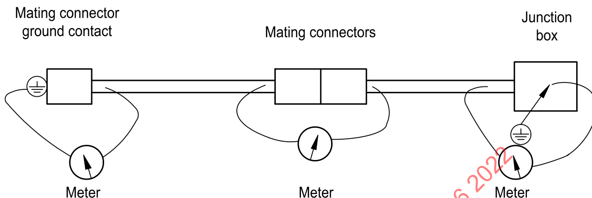
Figure 19.1 Grounding-Impedance test
