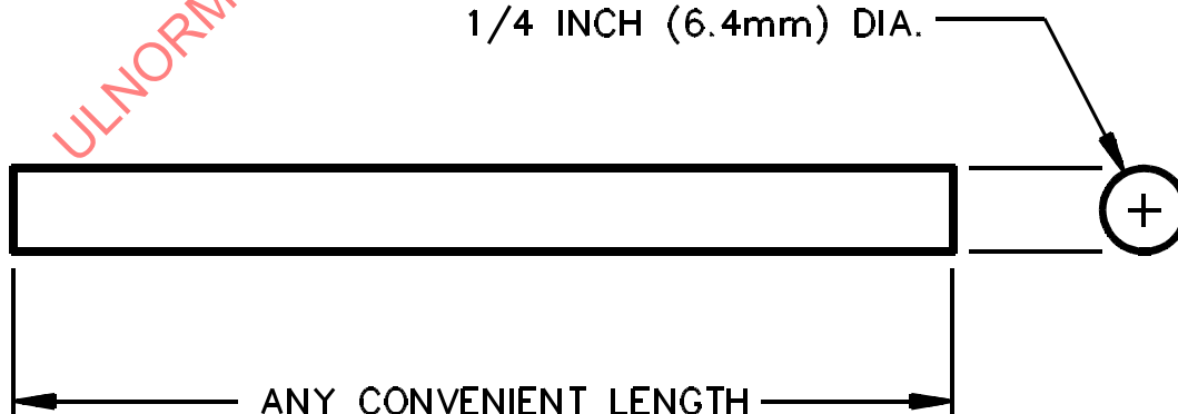
Figure 9.1 Accessibility probe
