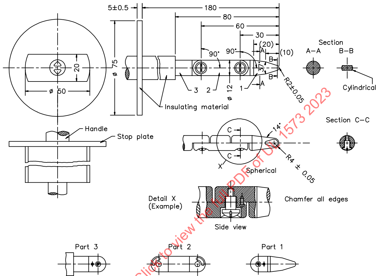
Figure 11.4 Articulate probe
