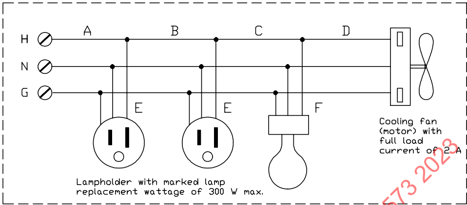
Figure 18.4 Illustrative example of requirements in 18.3.2
