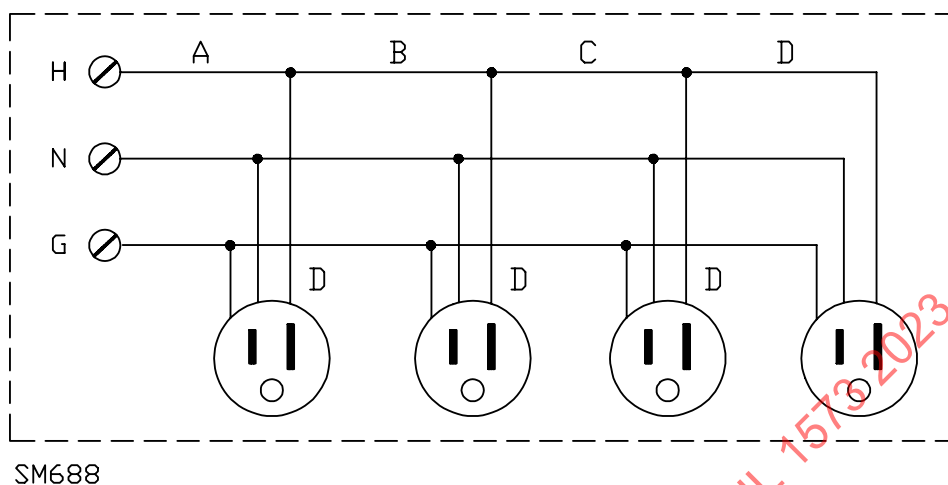
Figure 18.5 Illustrative example of requirements in 18.3.2
