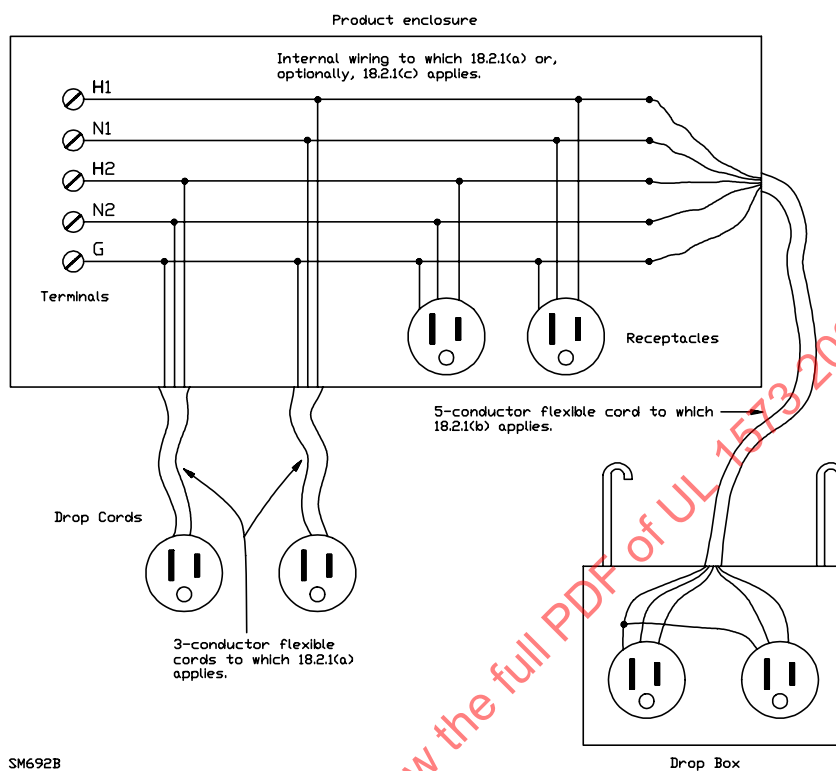
Figure 18.1 Illustrative example of requirements in 18.2.1
