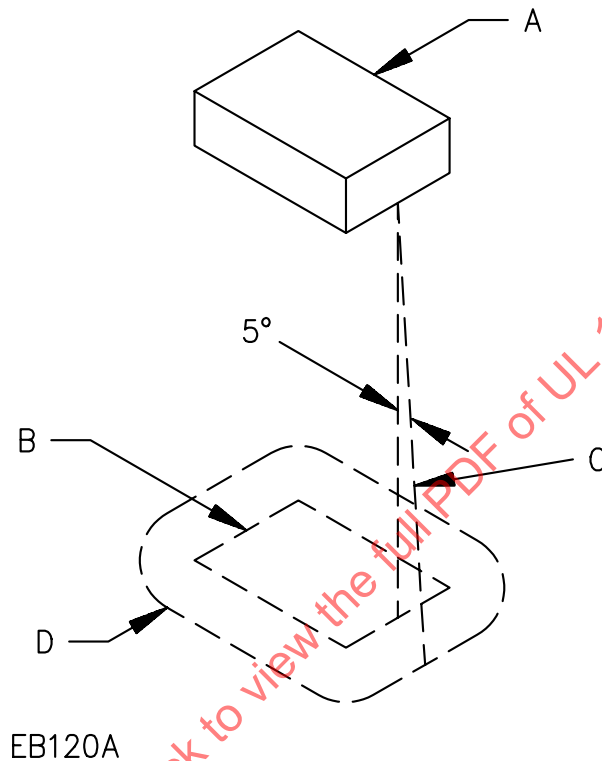
Figure 8.1 Location and extent of barrier
