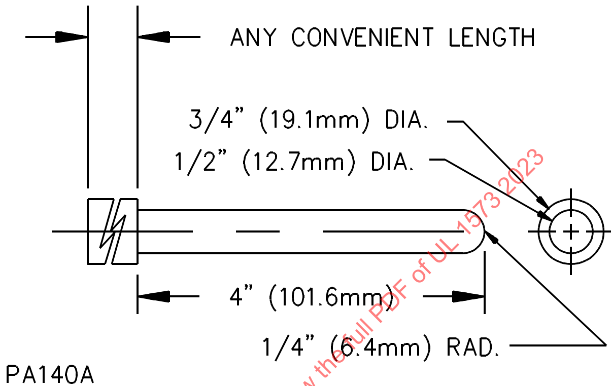
Figure 11.3 Probe for film-coated wire
