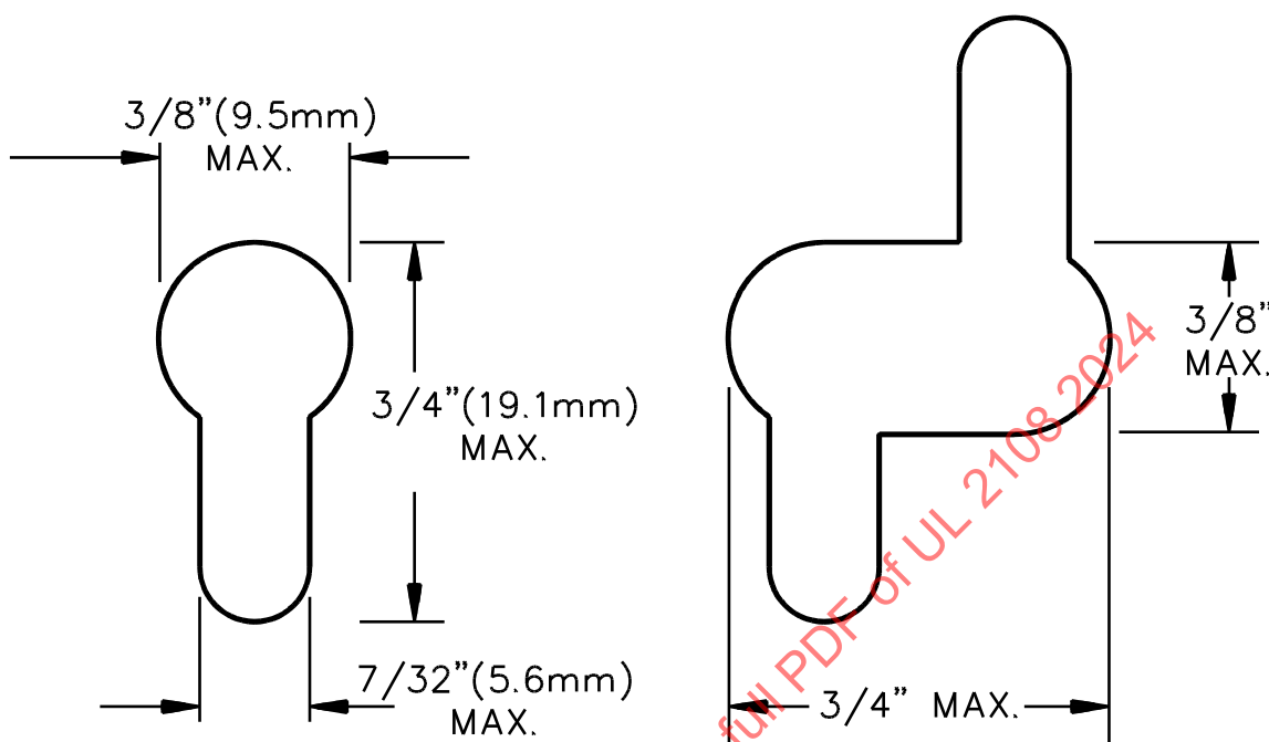
Figure 31.1 Keyhole slot/joined keyhole slot
