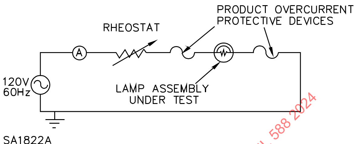
Figure 84.1 Cascade lamp burnout simulation circuit
