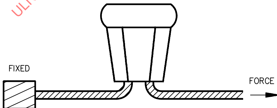
Figure 79.1 Application of pull
