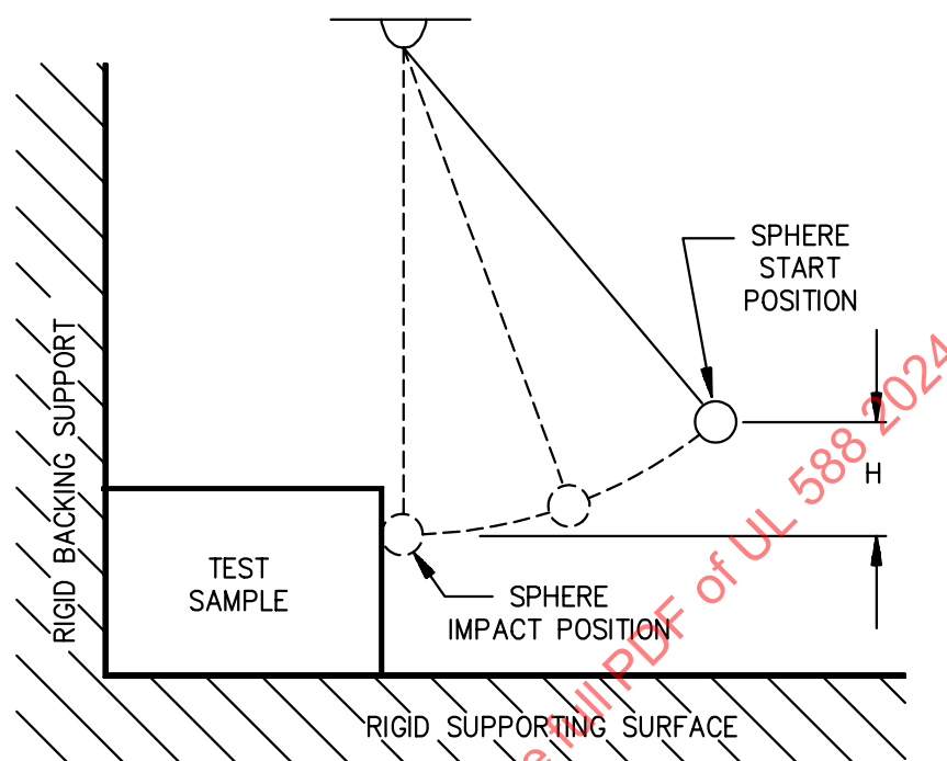
Figure 60.2 Ball pendulum impact test
