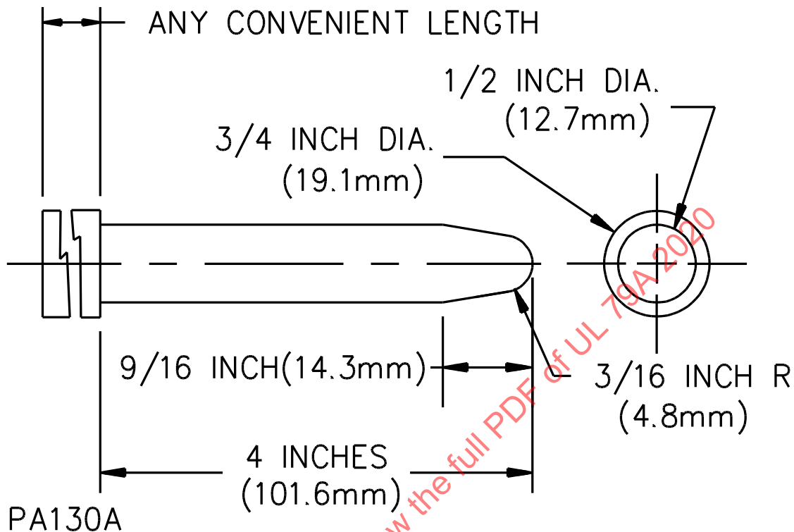
Figure 34.1 Accessibility probe for moving parts
