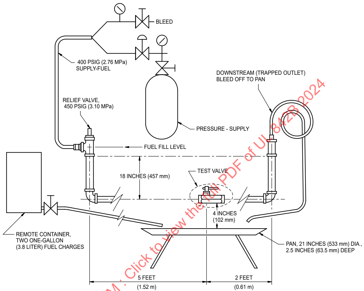
Figure 18.1 Test Configuration
