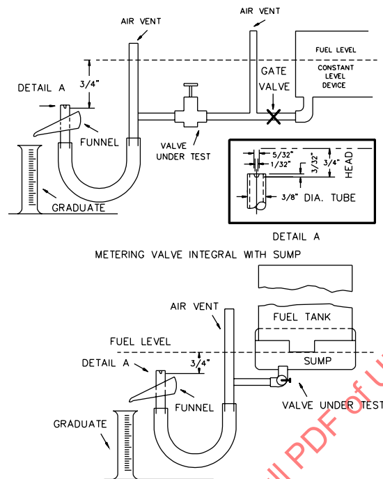
Figure 38.2 Flow rate test
