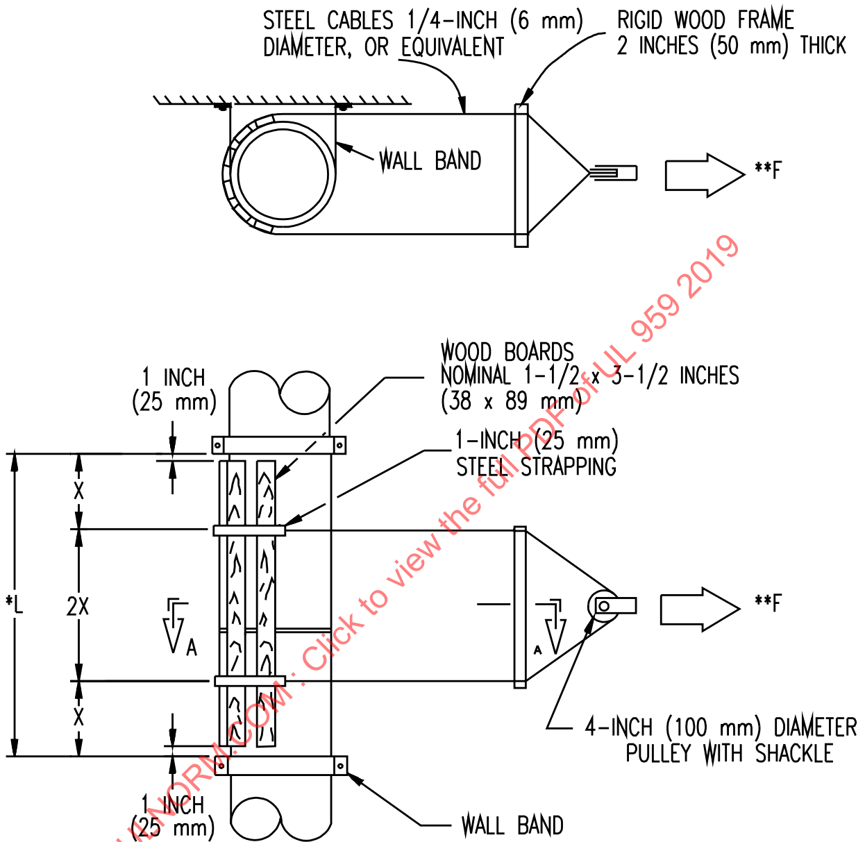
Figure 21.2 Wind load test for chimneys intended for exposed exterior installation
