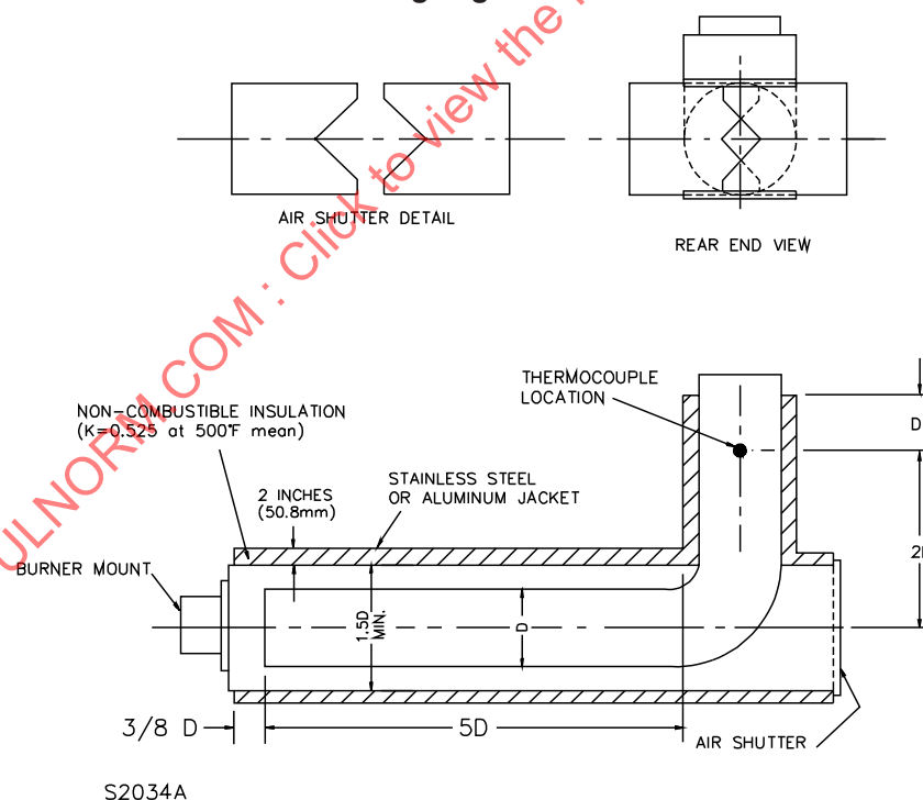
Figure 14.4 Flue-gas generator
