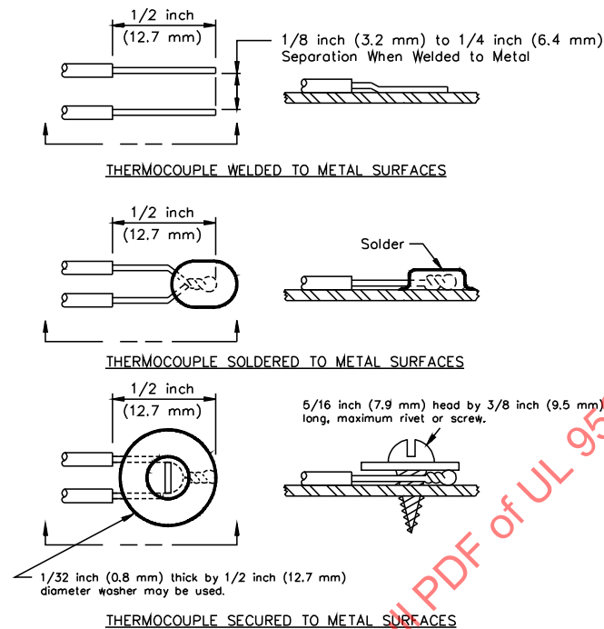
Figure 15.3 Thermocouple installation methods on metal surfaces
