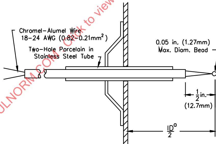
Figure 15.1 Flue-gas thermocouple and support bracket
