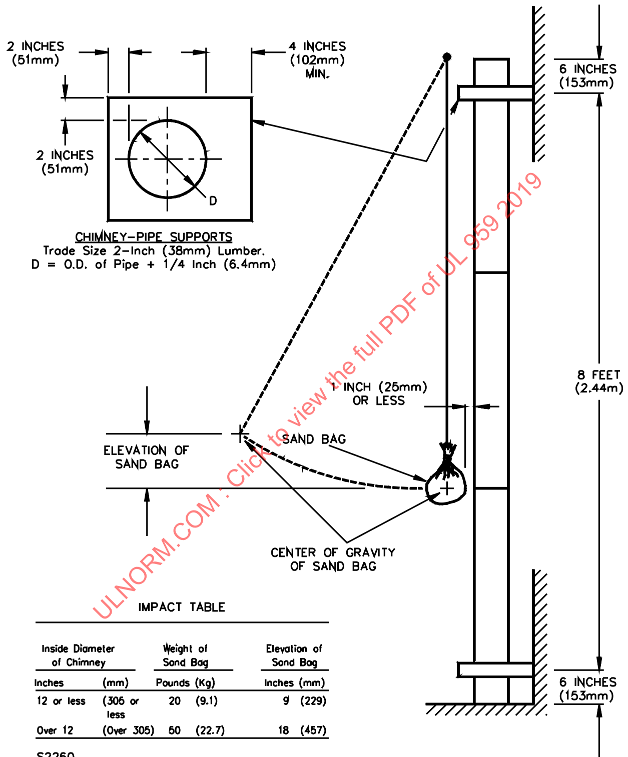
Figure 20.1 Strength test
