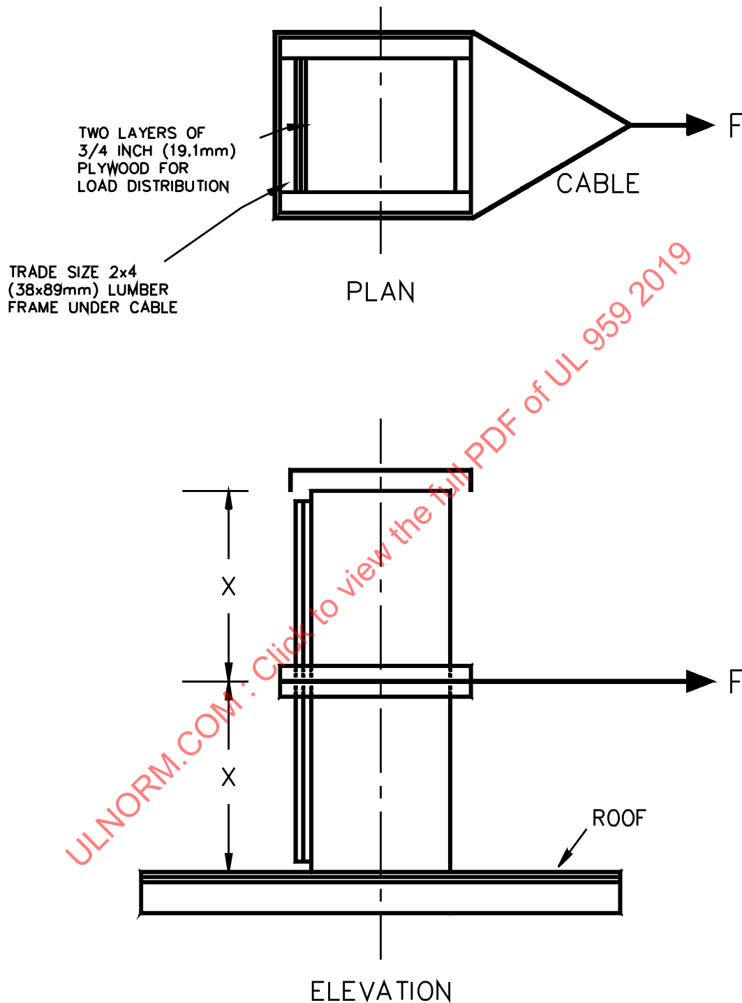
Figure 21.1 Wind load test on roof assembly
