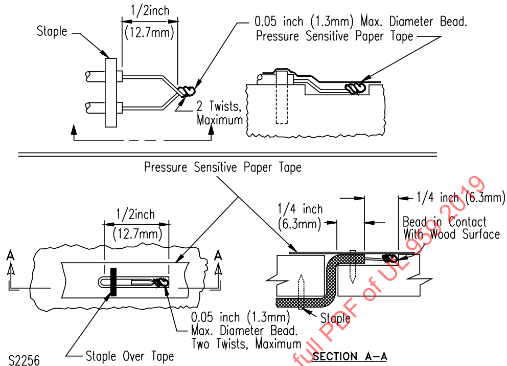
Figure 15.2 Thermocouple installation methods on wood surfaces
